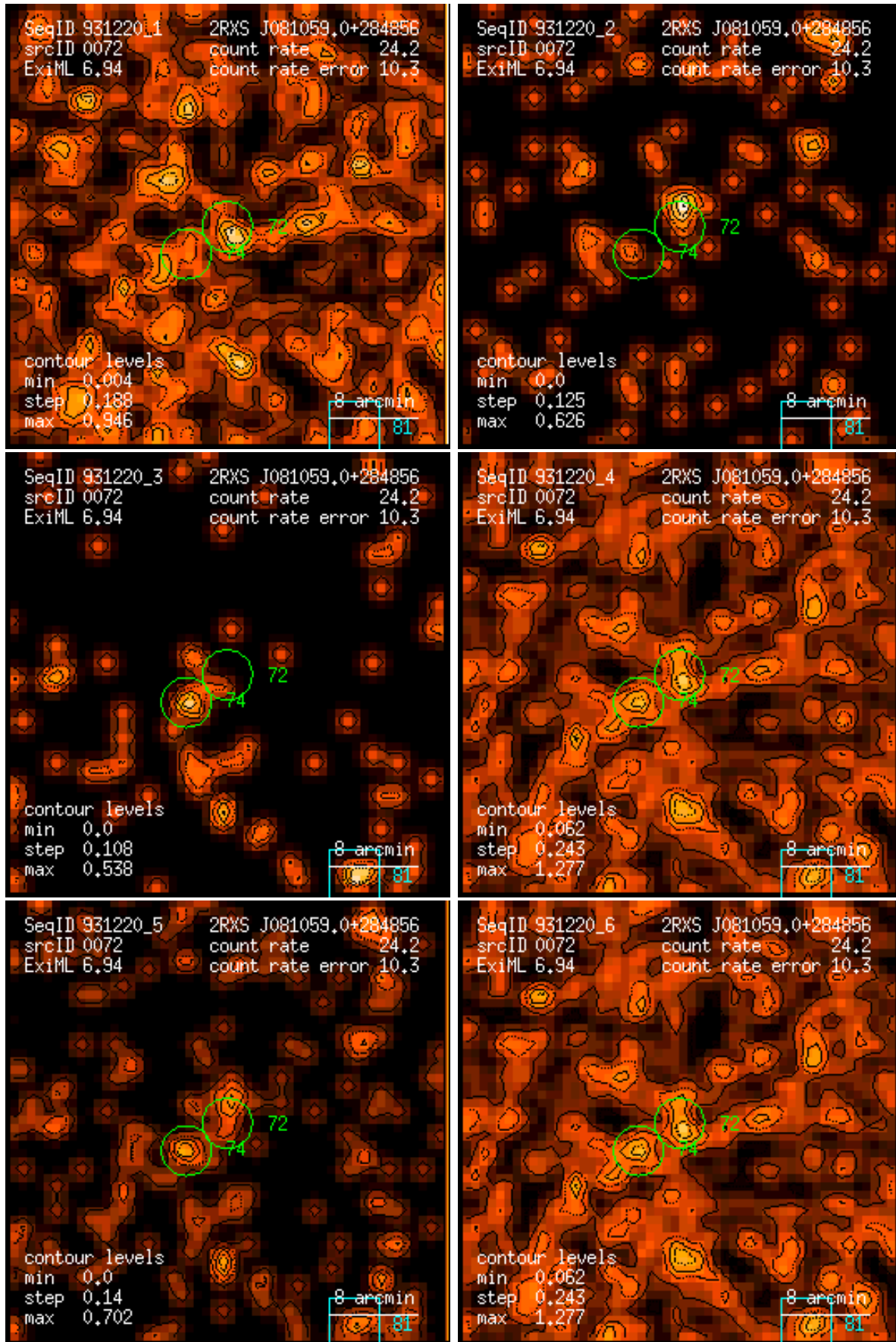
Figure 72: RASS 931220: detection 0072: band rate images, Gaussian filter: (1) PSPC channels 11 – 41, (2) 52 – 90, (3) 91 – 201, (4) 11 – 235, (5) 52 – 201, (6) 11 – 201. Broad band rates in counts/ks. Band rate contour levels in counts/ks/arcmin 2 .
