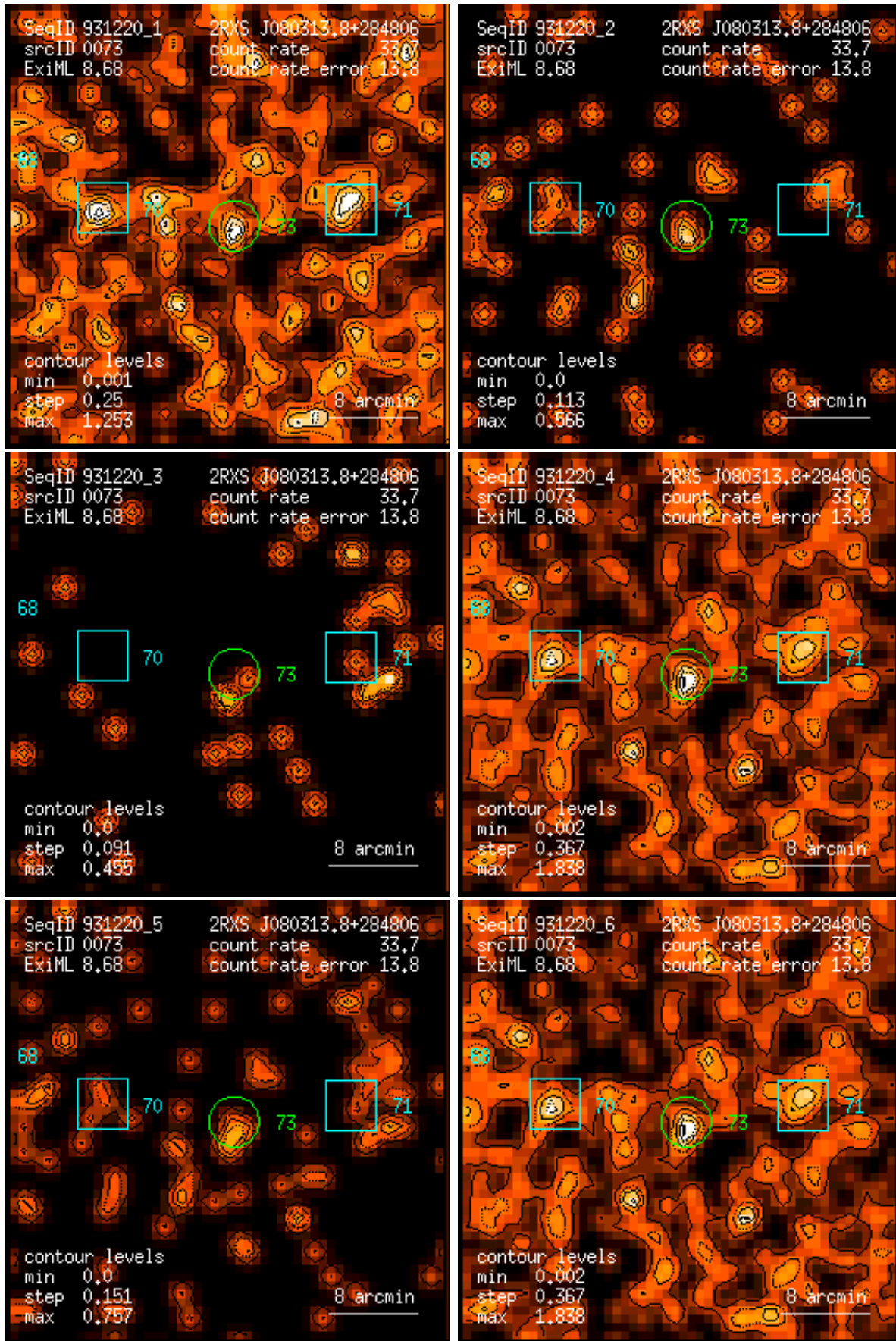
Figure 73: RASS 931220: detection 0073: band rate images, Gaussian filter: (1) PSPC channels 11 – 41, (2) 52 – 90, (3) 91 – 201, (4) 11 – 235, (5) 52 – 201, (6) 11 – 201. Broad band rates in counts/ks. Band rate contour levels in counts/ks/arcmin 2 .
