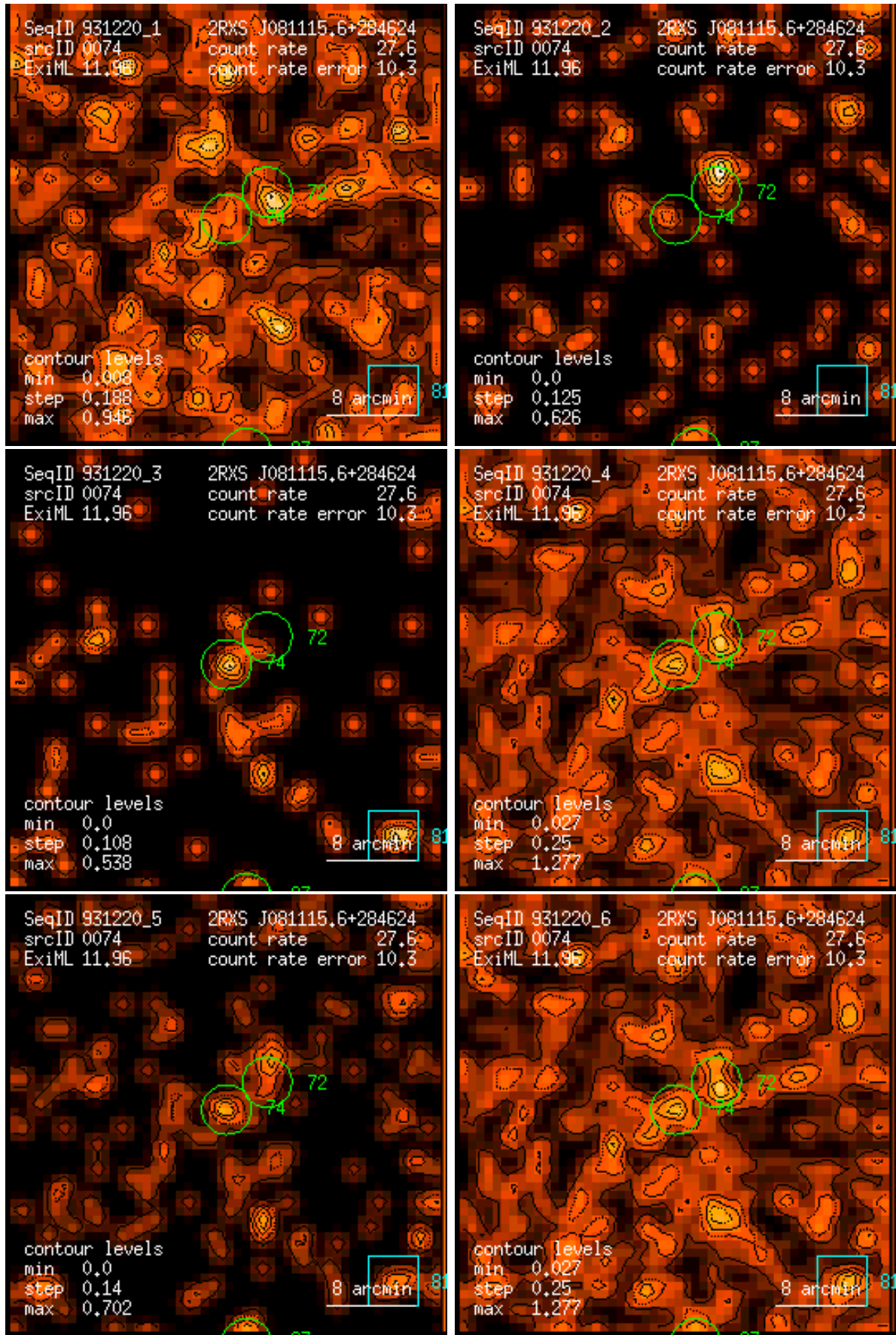
Figure 74: RASS 931220: detection 0074: band rate images, Gaussian filter: (1) PSPC channels 11 – 41, (2) 52 – 90, (3) 91 – 201, (4) 11 – 235, (5) 52 – 201, (6) 11 – 201. Broad band rates in counts/ks. Band rate contour levels in counts/ks/arcmin 2 .
