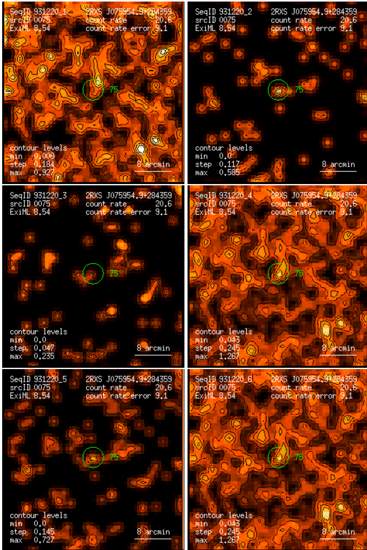
Figure 75: RASS 931220: detection 0075: band rate images, Gaussian filter: (1) PSPC channels 11 – 41, (2) 52 – 90, (3) 91 – 201, (4) 11 – 235, (5) 52 – 201, (6) 11 – 201. Broad band rates in counts/ks. Band rate contour levels in counts/ks/arcmin 2 .
