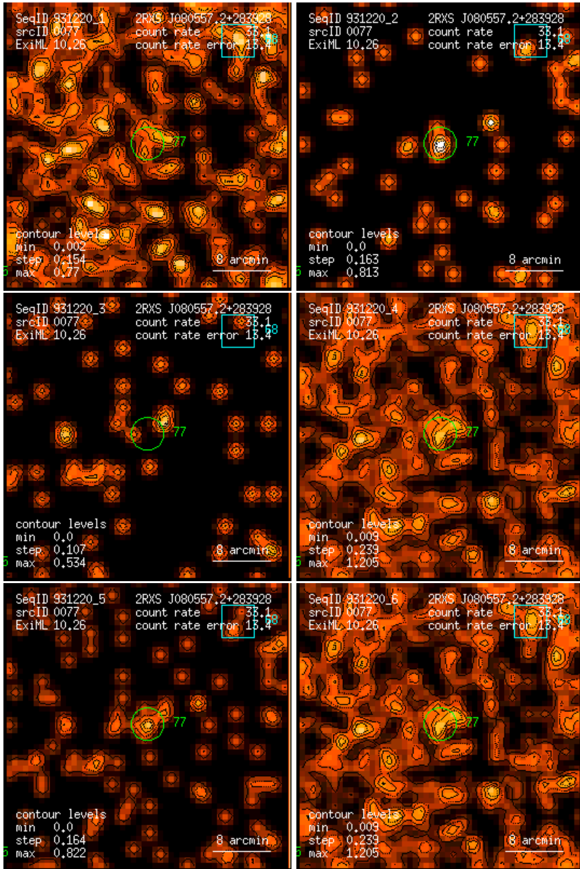
Figure 77: RASS 931220: detection 0077: band rate images, Gaussian filter: (1) PSPC channels 11 – 41, (2) 52 – 90, (3) 91 – 201, (4) 11 – 235, (5) 52 – 201, (6) 11 – 201. Broad band rates in counts/ks. Band rate contour levels in counts/ks/arcmin 2 .
