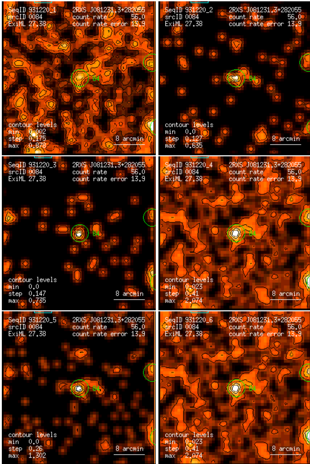
Figure 84: RASS 931220: detection 0084: band rate images, Gaussian filter: (1) PSPC channels 11 – 41, (2) 52 – 90, (3) 91 – 201, (4) 11 – 235, (5) 52 – 201, (6) 11 – 201. Broad band rates in counts/ks. Band rate contour levels in counts/ks/arcmin 2 .
