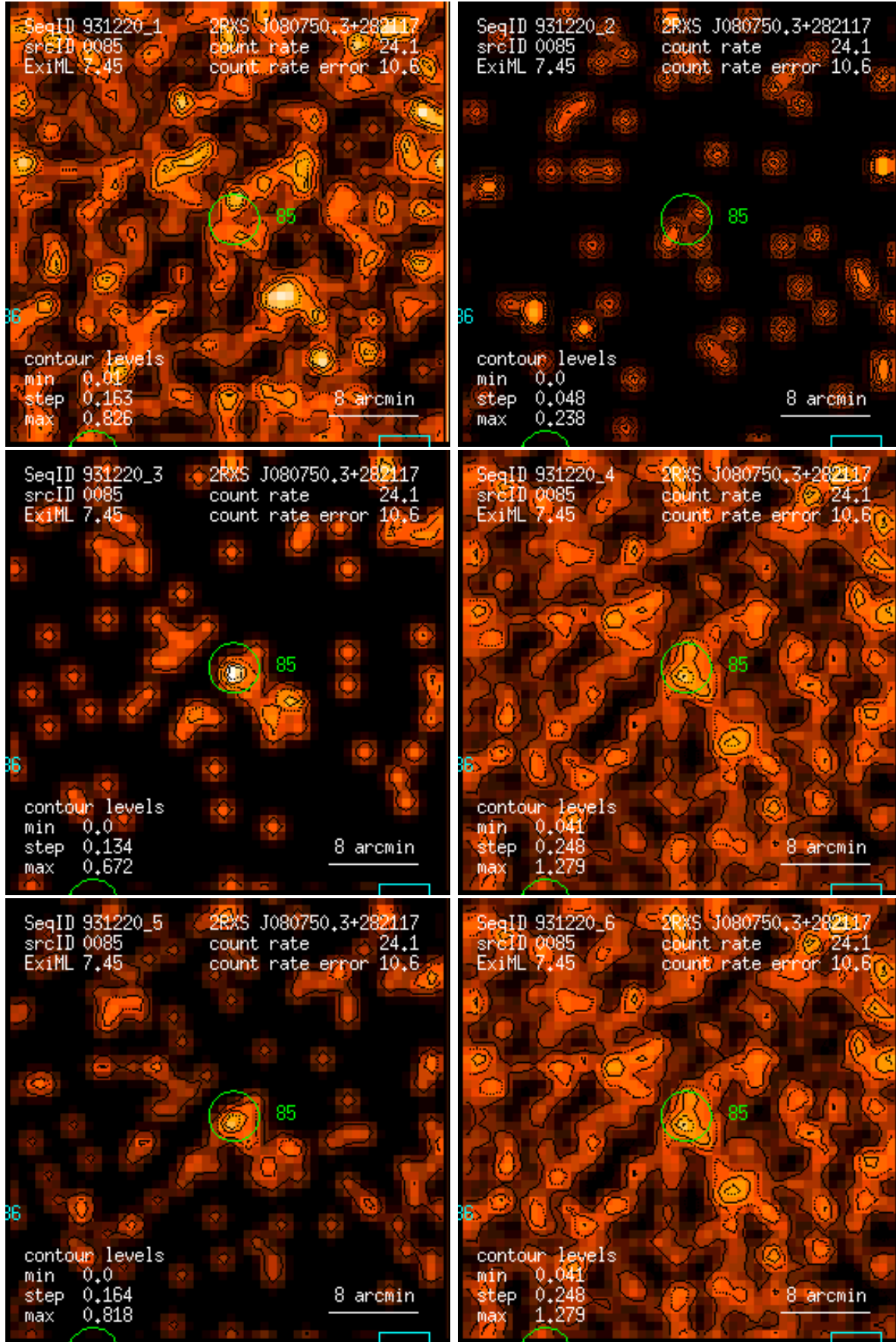
Figure 85: RASS 931220: detection 0085: band rate images, Gaussian filter: (1) PSPC channels 11 – 41, (2) 52 – 90, (3) 91 – 201, (4) 11 – 235, (5) 52 – 201, (6) 11 – 201. Broad band rates in counts/ks. Band rate contour levels in counts/ks/arcmin 2 .
