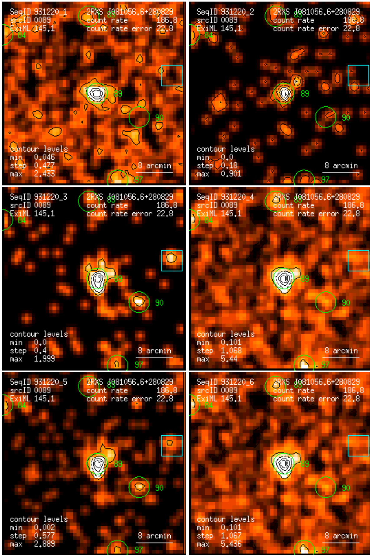
Figure 89: RASS 931220: detection 0089: band rate images, Gaussian filter: (1) PSPC channels 11 – 41, (2) 52 – 90, (3) 91 – 201, (4) 11 – 235, (5) 52 – 201, (6) 11 – 201. Broad band rates in counts/ks. Band rate contour levels in counts/ks/arcmin 2 .
