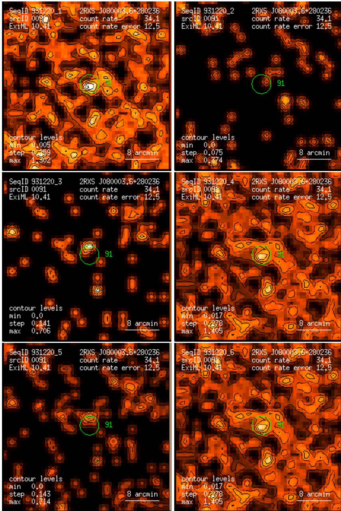
Figure 91: RASS 931220: detection 0091: band rate images, Gaussian filter: (1) PSPC channels 11 – 41, (2) 52 – 90, (3) 91 – 201, (4) 11 – 235, (5) 52 – 201, (6) 11 – 201. Broad band rates in counts/ks. Band rate contour levels in counts/ks/arcmin 2 .
