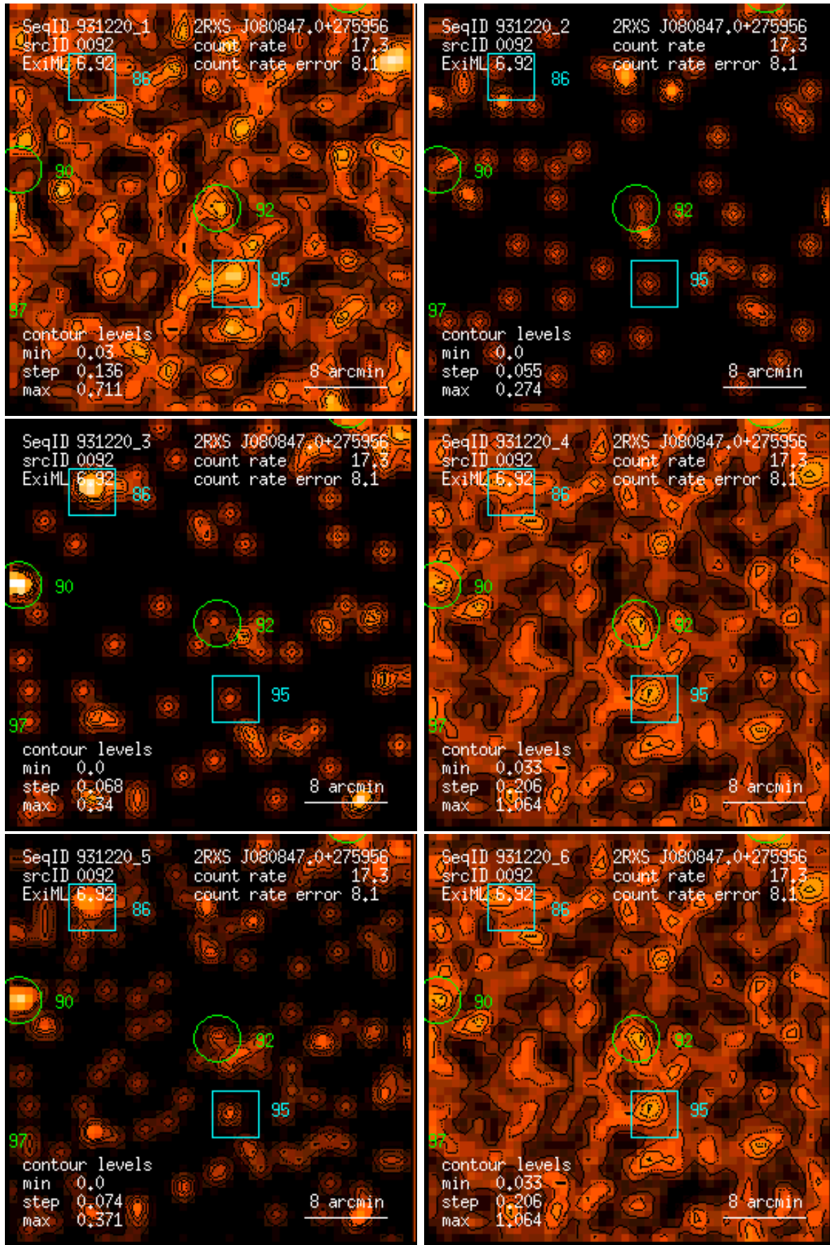
Figure 92: RASS 931220: detection 0092: band rate images, Gaussian filter: (1) PSPC channels 11 – 41, (2) 52 – 90, (3) 91 – 201, (4) 11 – 235, (5) 52 – 201, (6) 11 – 201. Broad band rates in counts/ks. Band rate contour levels in counts/ks/arcmin 2 .
