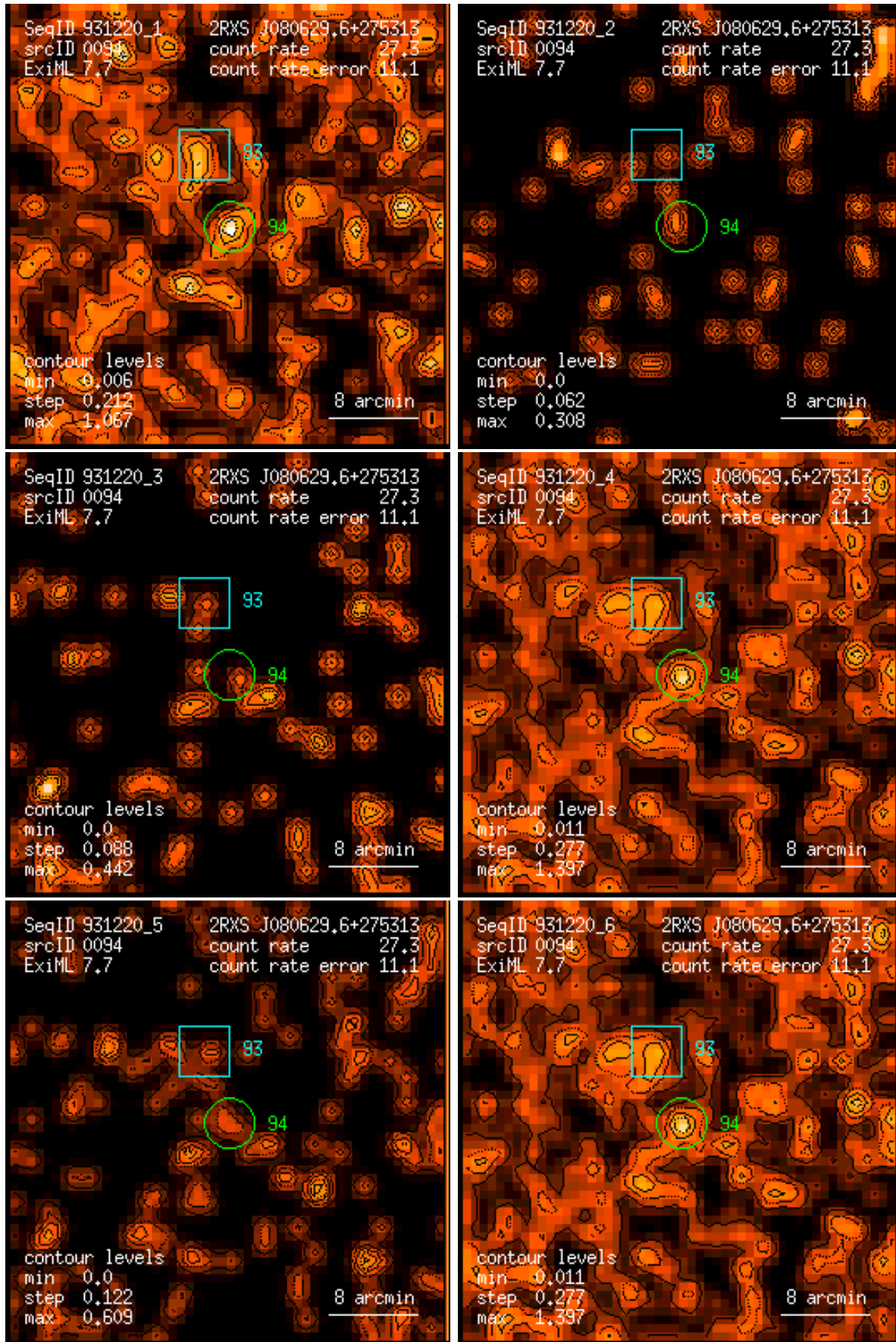
Figure 94: RASS 931220: detection 0094: band rate images, Gaussian filter: (1) PSPC channels 11 – 41, (2) 52 – 90, (3) 91 – 201, (4) 11 – 235, (5) 52 – 201, (6) 11 – 201. Broad band rates in counts/ks. Band rate contour levels in counts/ks/arcmin 2 .
