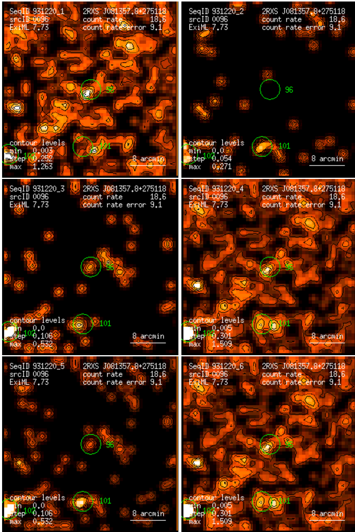
Figure 96: RASS 931220: detection 0096: band rate images, Gaussian filter: (1) PSPC channels 11 – 41, (2) 52 – 90, (3) 91 – 201, (4) 11 – 235, (5) 52 – 201, (6) 11 – 201. Broad band rates in counts/ks. Band rate contour levels in counts/ks/arcmin 2 .
