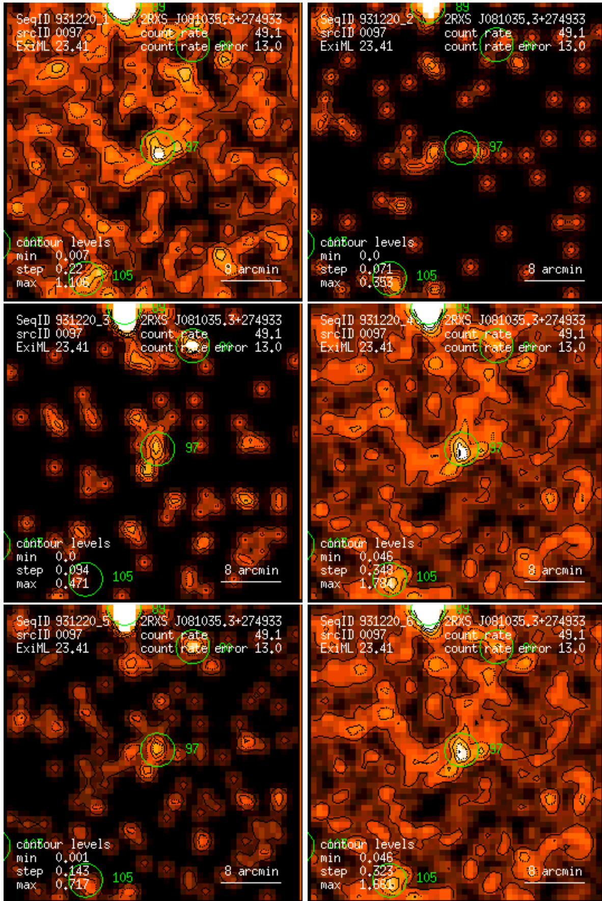
Figure 97: RASS 931220: detection 0097: band rate images, Gaussian filter: (1) PSPC channels 11 – 41, (2) 52 – 90, (3) 91 – 201, (4) 11 – 235, (5) 52 – 201, (6) 11 – 201. Broad band rates in counts/ks. Band rate contour levels in counts/ks/arcmin 2 .
