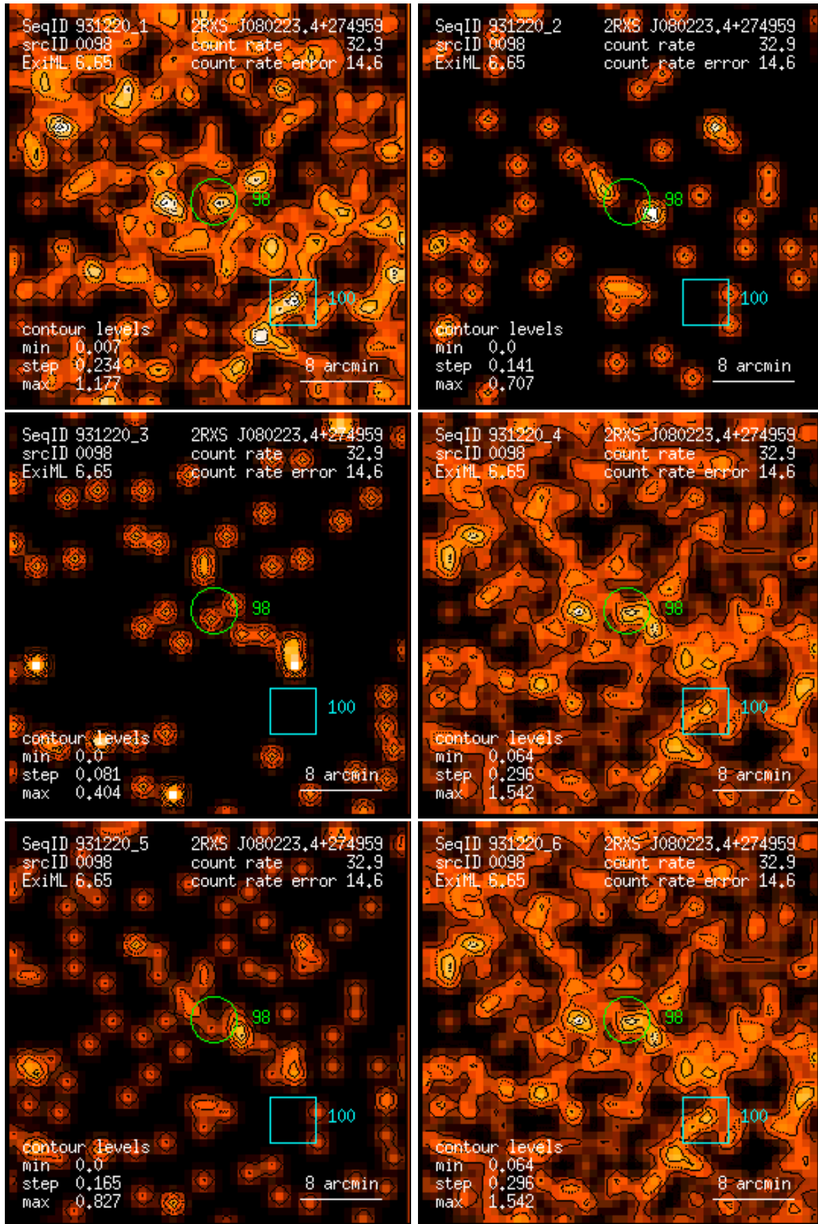
Figure 98: RASS 931220: detection 0098: band rate images, Gaussian filter: (1) PSPC channels 11 – 41, (2) 52 – 90, (3) 91 – 201, (4) 11 – 235, (5) 52 – 201, (6) 11 – 201. Broad band rates in counts/ks. Band rate contour levels in counts/ks/arcmin 2 .
