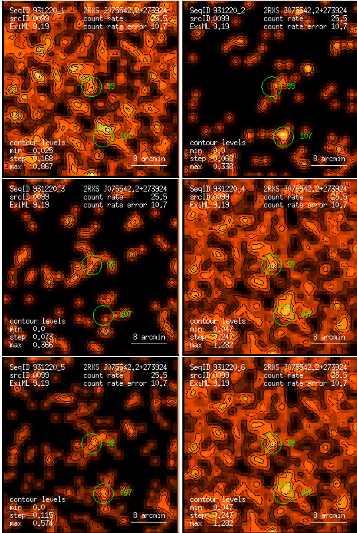
Figure 99: RASS 931220: detection 0099: band rate images, Gaussian filter: (1) PSPC channels 11 – 41, (2) 52 – 90, (3) 91 – 201, (4) 11 – 235, (5) 52 – 201, (6) 11 – 201. Broad band rates in counts/ks. Band rate contour levels in counts/ks/arcmin 2 .
