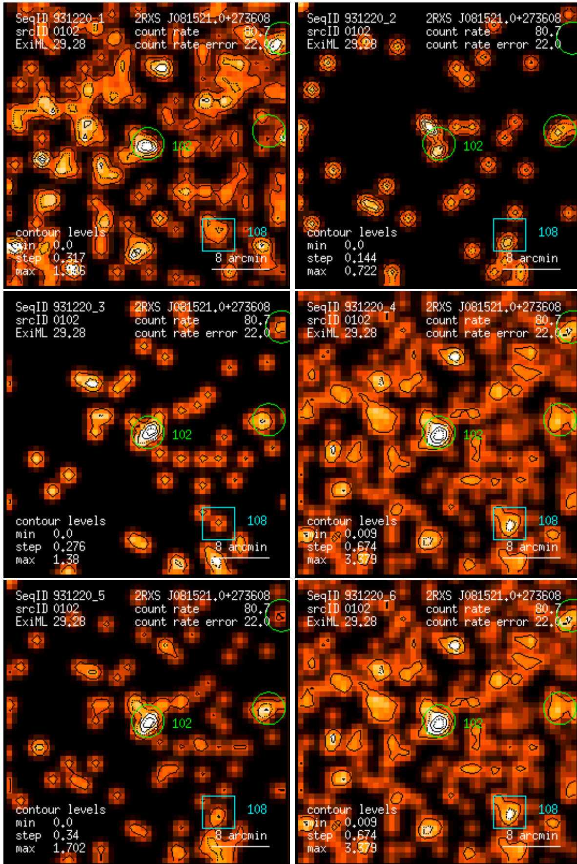
Figure 102: RASS 931220: detection 0102: band rate images, Gaussian filter: (1) PSPC channels 11 – 41, (2) 52 – 90, (3) 91 – 201, (4) 11 – 235, (5) 52 – 201, (6) 11 – 201. Broad band rates in counts/ks. Band rate contour levels in counts/ks/arcmin 2 .
