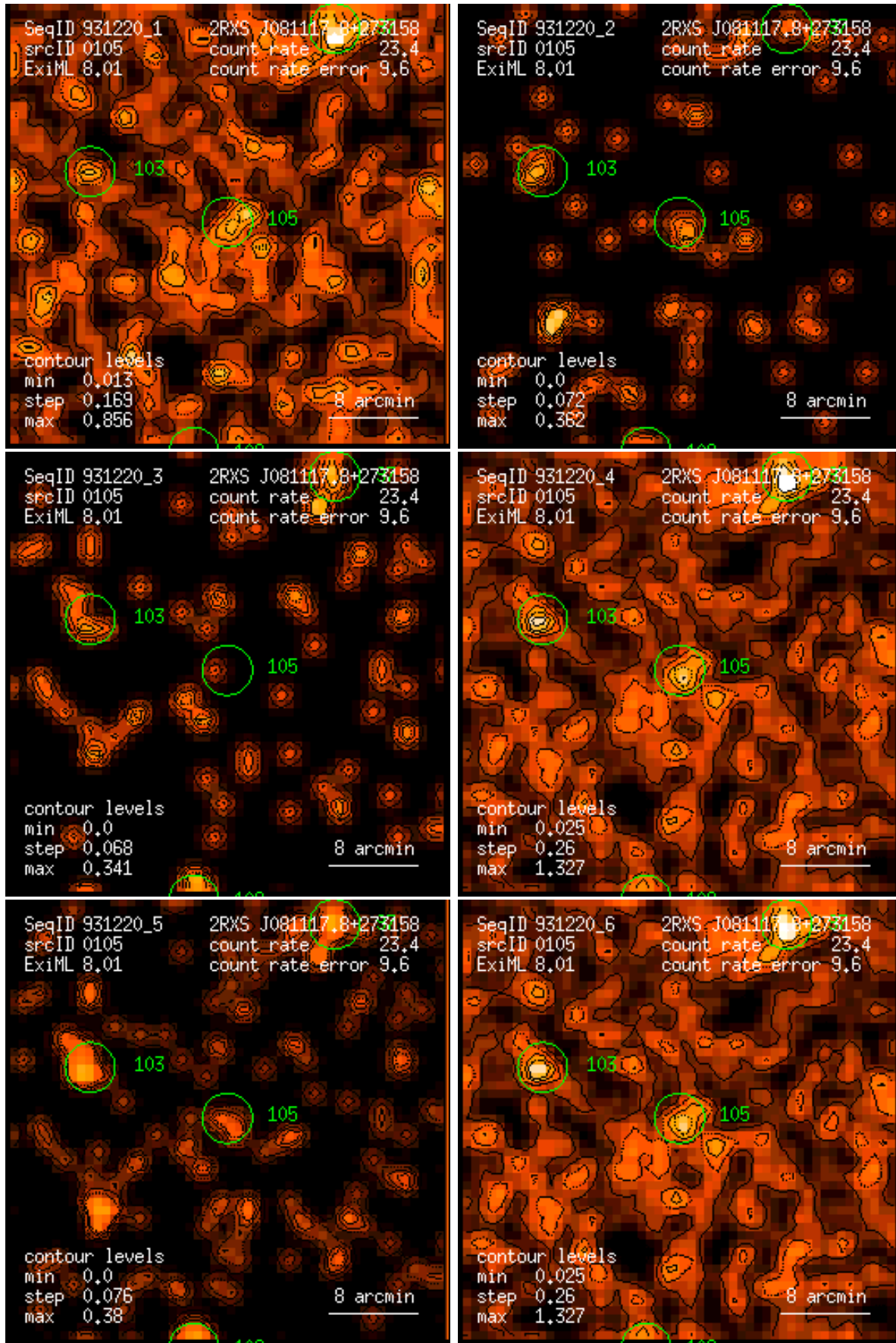
Figure 105: RASS 931220: detection 0105: band rate images, Gaussian filter: (1) PSPC channels 11 – 41, (2) 52 – 90, (3) 91 – 201, (4) 11 – 235, (5) 52 – 201, (6) 11 – 201. Broad band rates in counts/ks. Band rate contour levels in counts/ks/arcmin 2 .
