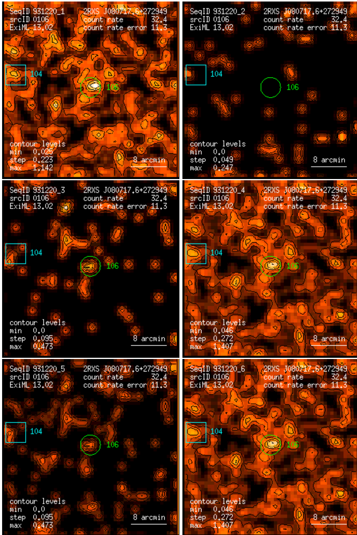
Figure 106: RASS 931220: detection 0106: band rate images, Gaussian filter: (1) PSPC channels 11 – 41, (2) 52 – 90, (3) 91 – 201, (4) 11 – 235, (5) 52 – 201, (6) 11 – 201. Broad band rates in counts/ks. Band rate contour levels in counts/ks/arcmin 2 .
