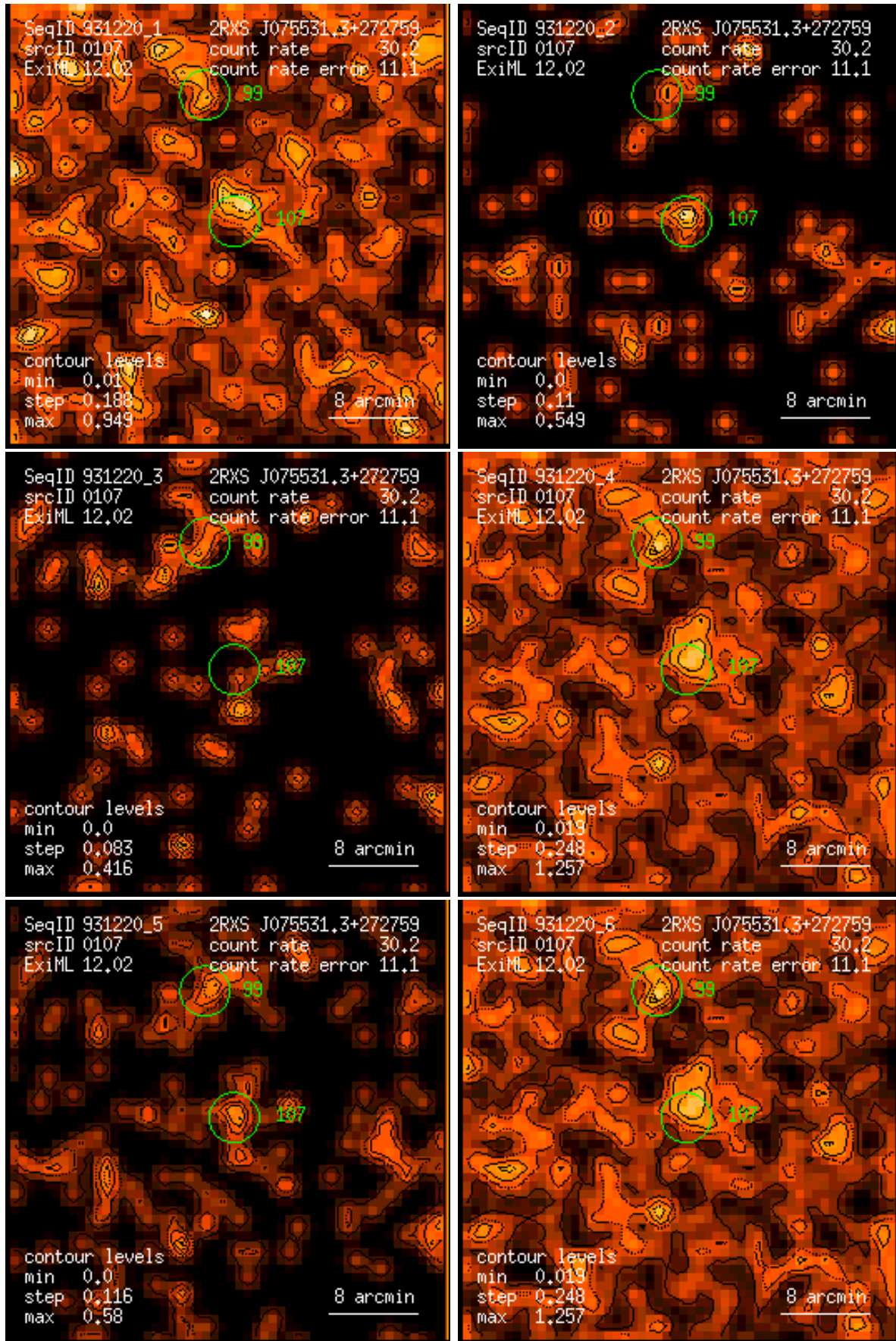
Figure 107: RASS 931220: detection 0107: band rate images, Gaussian filter: (1) PSPC channels 11 – 41, (2) 52 – 90, (3) 91 – 201, (4) 11 – 235, (5) 52 – 201, (6) 11 – 201. Broad band rates in counts/ks. Band rate contour levels in counts/ks/arcmin 2 .
