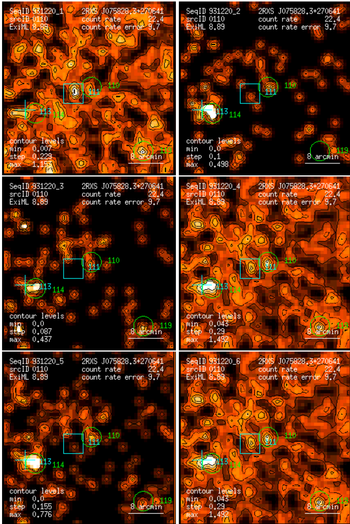
Figure 110: RASS 931220: detection 0110: band rate images, Gaussian filter: (1) PSPC channels 11 – 41, (2) 52 – 90, (3) 91 – 201, (4) 11 – 235, (5) 52 – 201, (6) 11 – 201. Broad band rates in counts/ks. Band rate contour levels in counts/ks/arcmin 2 .
