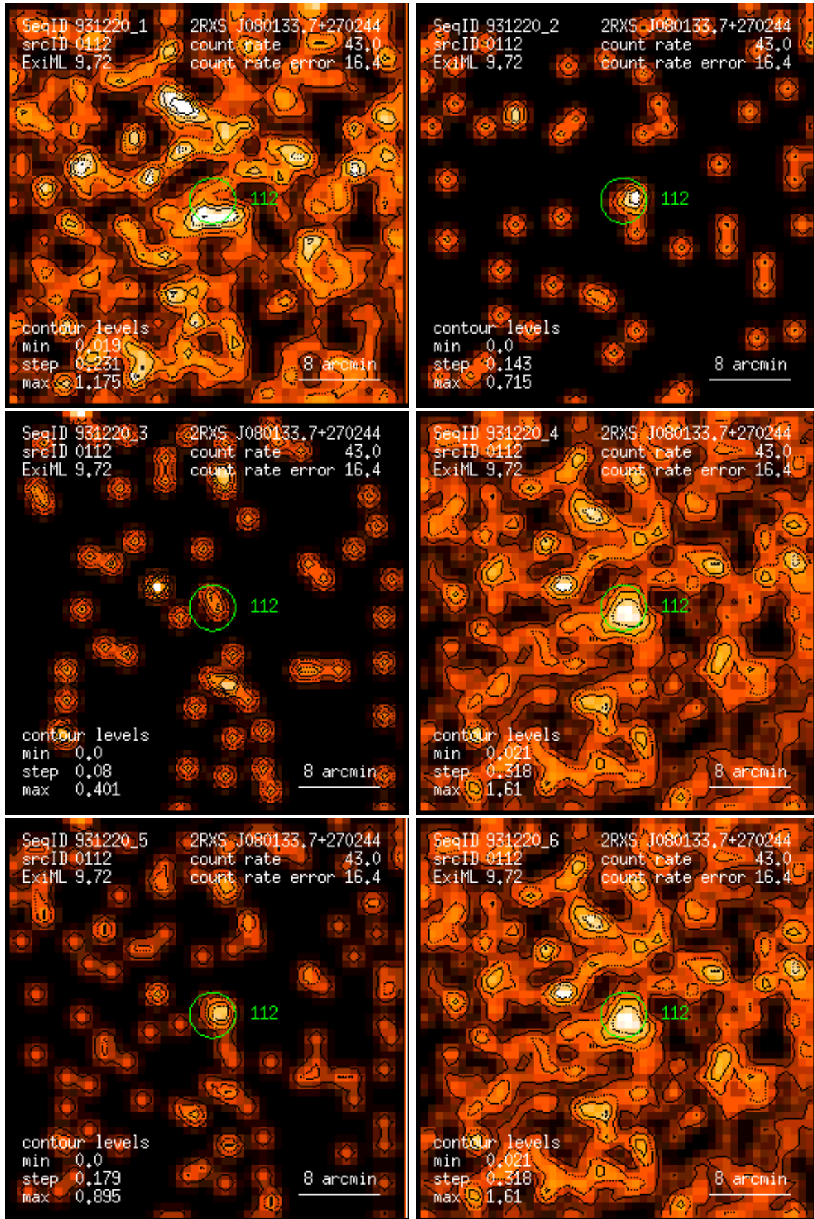
Figure 112: RASS 931220: detection 0112: band rate images, Gaussian filter: (1) PSPC channels 11 – 41, (2) 52 – 90, (3) 91 – 201, (4) 11 – 235, (5) 52 – 201, (6) 11 – 201. Broad band rates in counts/ks. Band rate contour levels in counts/ks/arcmin 2 .
