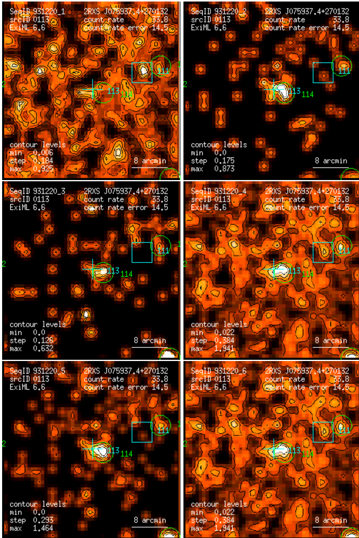
Figure 113: RASS 931220: detection 0113: band rate images, Gaussian filter: (1) PSPC channels 11 – 41, (2) 52 – 90, (3) 91 – 201, (4) 11 – 235, (5) 52 – 201, (6) 11 – 201. Broad band rates in counts/ks. Band rate contour levels in counts/ks/arcmin 2 .
