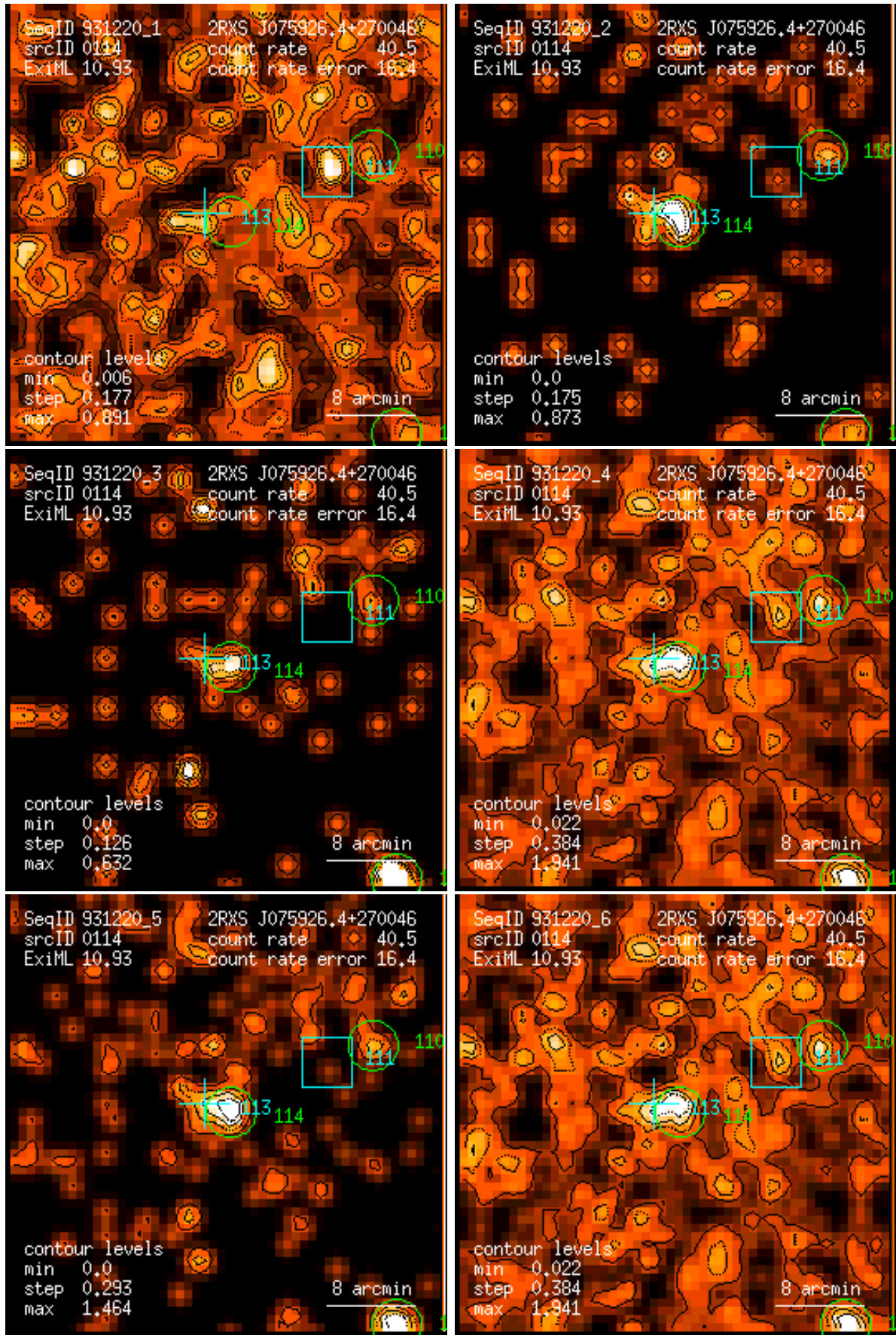
Figure 114: RASS 931220: detection 0114: band rate images, Gaussian filter: (1) PSPC channels 11 – 41, (2) 52 – 90, (3) 91 – 201, (4) 11 – 235, (5) 52 – 201, (6) 11 – 201. Broad band rates in counts/ks. Band rate contour levels in counts/ks/arcmin 2 .
