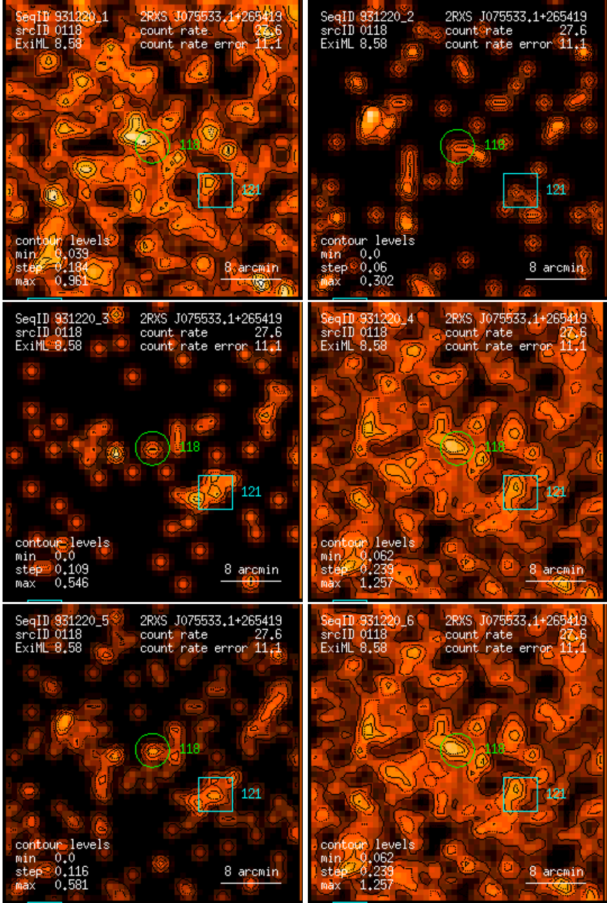
Figure 118: RASS 931220: detection 0118: band rate images, Gaussian filter: (1) PSPC channels 11 – 41, (2) 52 – 90, (3) 91 – 201, (4) 11 – 235, (5) 52 – 201, (6) 11 – 201. Broad band rates in counts/ks. Band rate contour levels in counts/ks/arcmin 2 .
