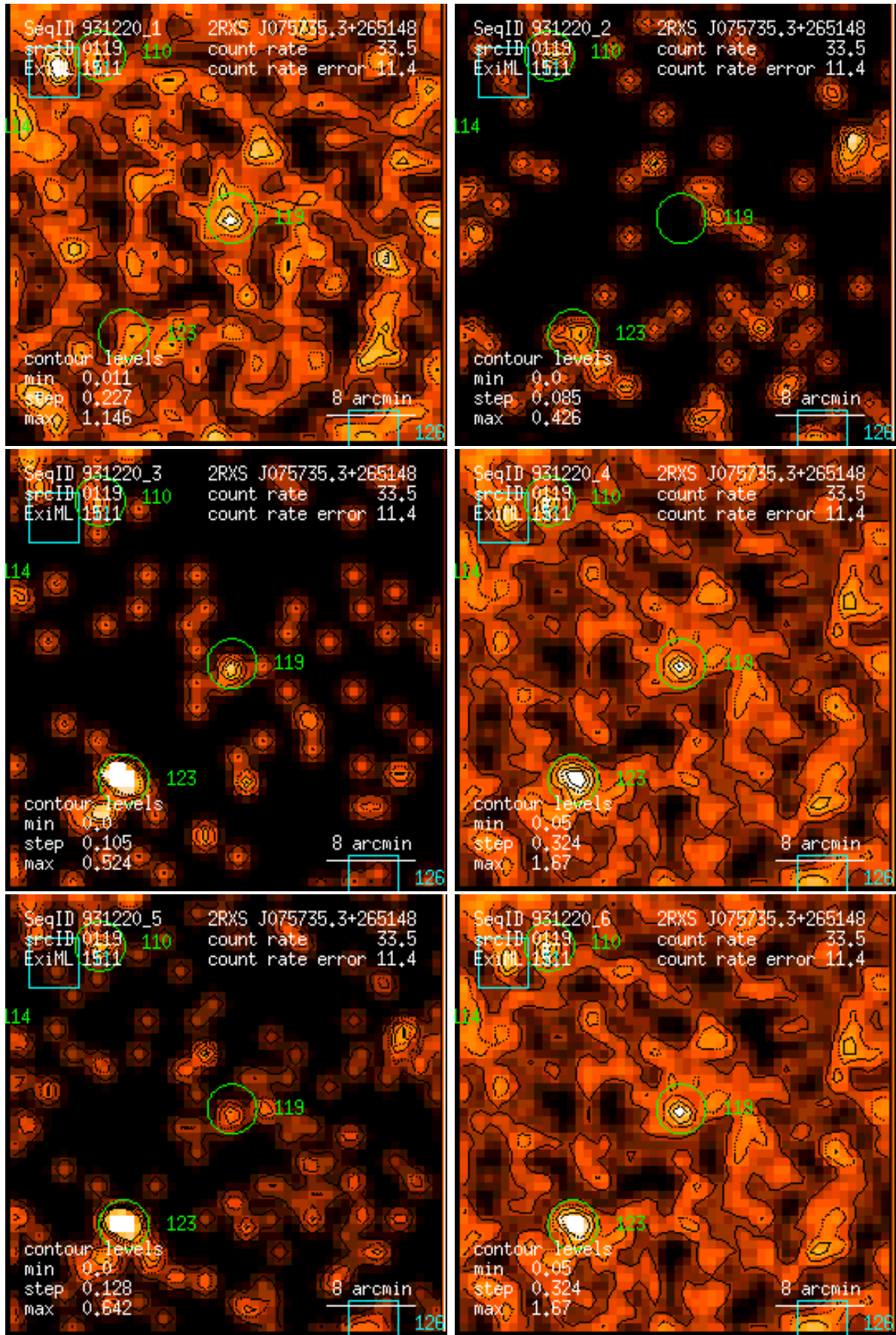
Figure 119: RASS 931220: detection 0119: band rate images, Gaussian filter: (1) PSPC channels 11 – 41, (2) 52 – 90, (3) 91 – 201, (4) 11 – 235, (5) 52 – 201, (6) 11 – 201. Broad band rates in counts/ks. Band rate contour levels in counts/ks/arcmin 2 .
