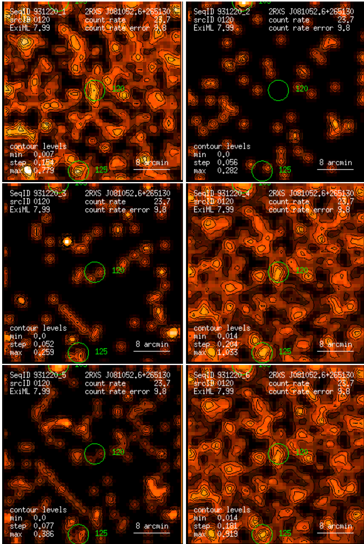
Figure 120: RASS 931220: detection 0120: band rate images, Gaussian filter: (1) PSPC channels 11 – 41, (2) 52 – 90, (3) 91 – 201, (4) 11 – 235, (5) 52 – 201, (6) 11 – 201. Broad band rates in counts/ks. Band rate contour levels in counts/ks/arcmin 2 .
