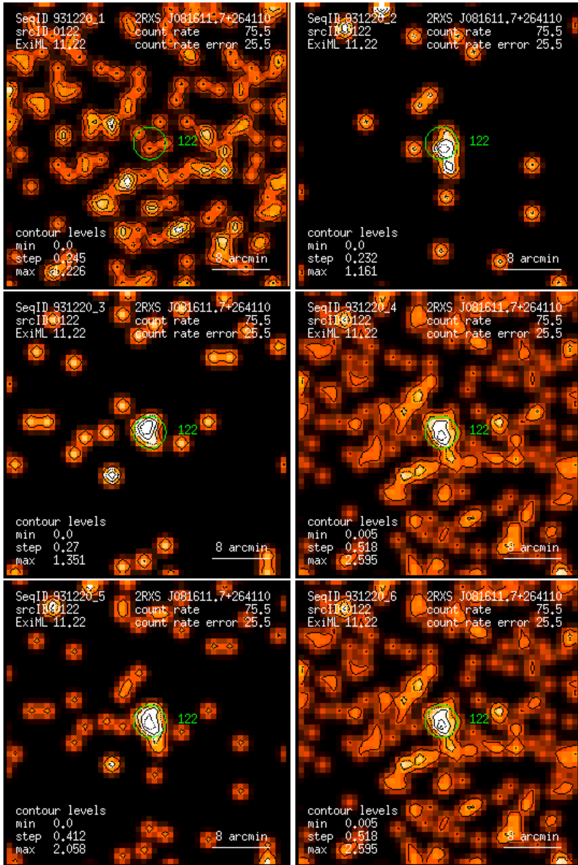
Figure 122: RASS 931220: detection 0122: band rate images, Gaussian filter: (1) PSPC channels 11 – 41, (2) 52 – 90, (3) 91 – 201, (4) 11 – 235, (5) 52 – 201, (6) 11 – 201. Broad band rates in counts/ks. Band rate contour levels in counts/ks/arcmin 2 .
