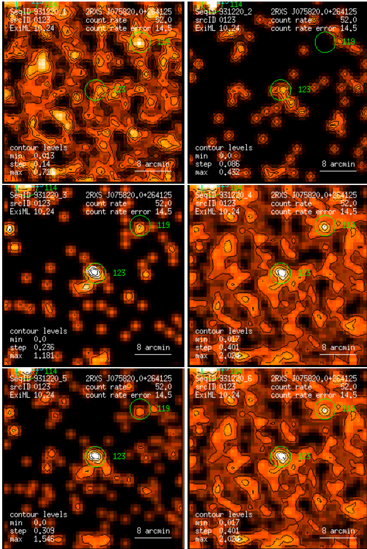
Figure 123: RASS 931220: detection 0123: band rate images, Gaussian filter: (1) PSPC channels 11 – 41, (2) 52 – 90, (3) 91 – 201, (4) 11 – 235, (5) 52 – 201, (6) 11 – 201. Broad band rates in counts/ks. Band rate contour levels in counts/ks/arcmin 2 .
