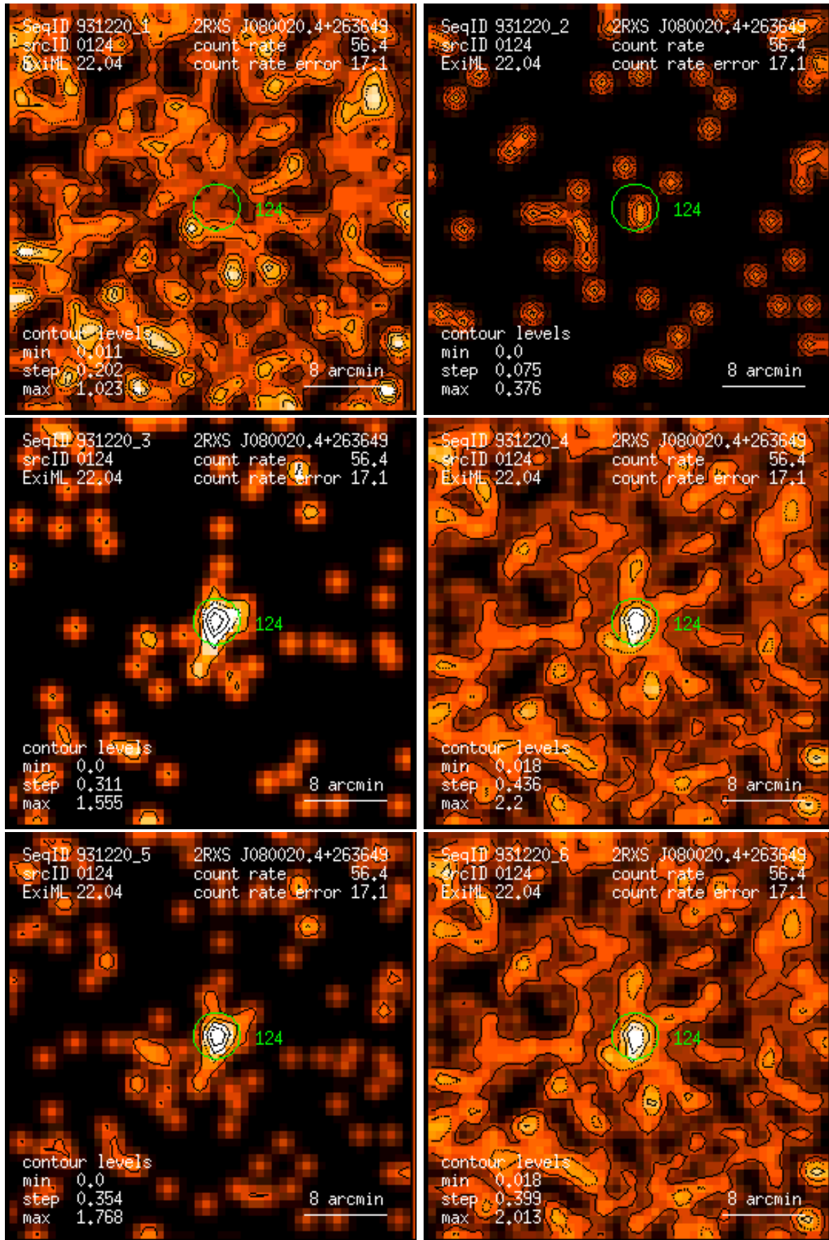
Figure 124: RASS 931220: detection 0124: band rate images, Gaussian filter: (1) PSPC channels 11 – 41, (2) 52 – 90, (3) 91 – 201, (4) 11 – 235, (5) 52 – 201, (6) 11 – 201. Broad band rates in counts/ks. Band rate contour levels in counts/ks/arcmin 2 .
