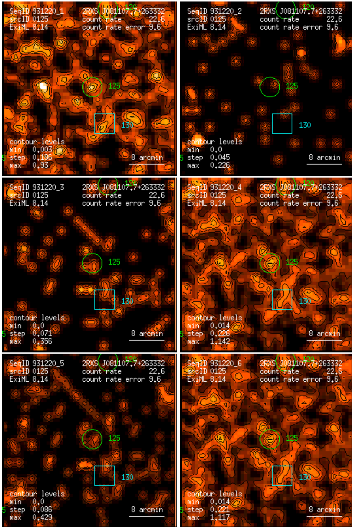
Figure 125: RASS 931220: detection 0125: band rate images, Gaussian filter: (1) PSPC channels 11 – 41, (2) 52 – 90, (3) 91 – 201, (4) 11 – 235, (5) 52 – 201, (6) 11 – 201. Broad band rates in counts/ks. Band rate contour levels in counts/ks/arcmin 2 .
