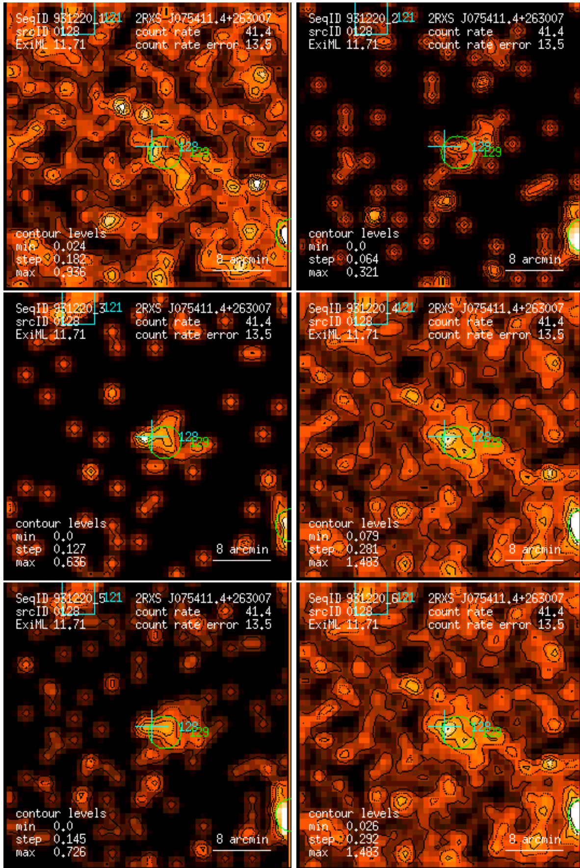
Figure 128: RASS 931220: detection 0128: band rate images, Gaussian filter: (1) PSPC channels 11 – 41, (2) 52 – 90, (3) 91 – 201, (4) 11 – 235, (5) 52 – 201, (6) 11 – 201. Broad band rates in counts/ks. Band rate contour levels in counts/ks/arcmin 2 .
