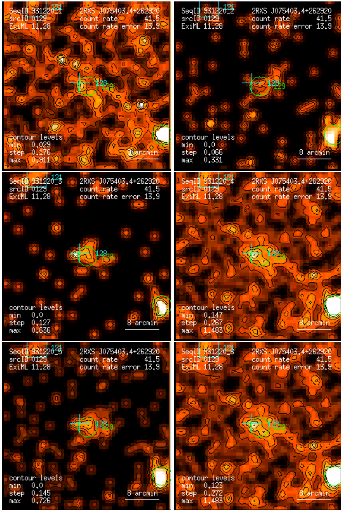
Figure 129: RASS 931220: detection 0129: band rate images, Gaussian filter: (1) PSPC channels 11 – 41, (2) 52 – 90, (3) 91 – 201, (4) 11 – 235, (5) 52 – 201, (6) 11 – 201. Broad band rates in counts/ks. Band rate contour levels in counts/ks/arcmin 2 .
