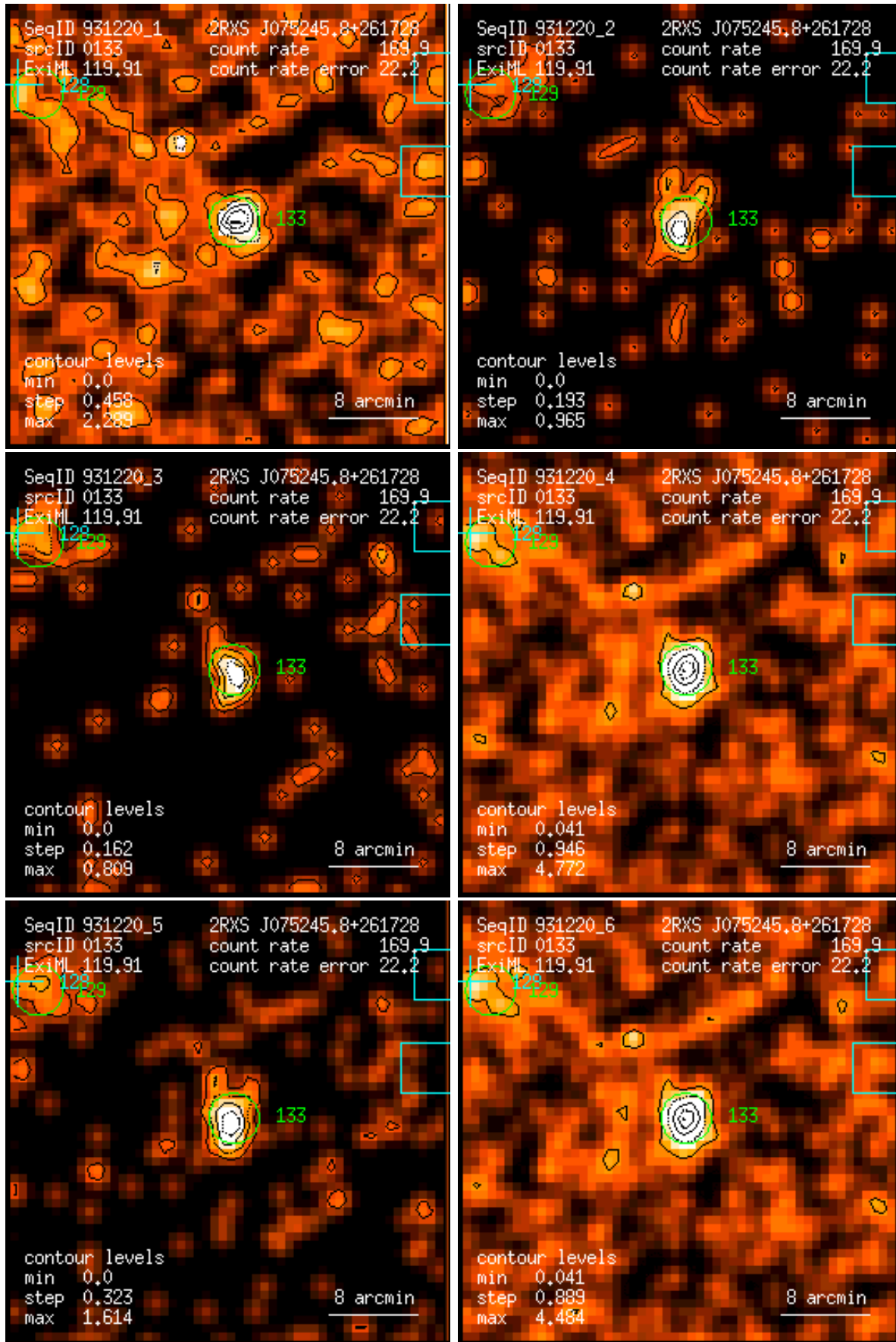
Figure 133: RASS 931220: detection 0133: band rate images, Gaussian filter: (1) PSPC channels 11 – 41, (2) 52 – 90, (3) 91 – 201, (4) 11 – 235, (5) 52 – 201, (6) 11 – 201. Broad band rates in counts/ks. Band rate contour levels in counts/ks/arcmin 2 .
