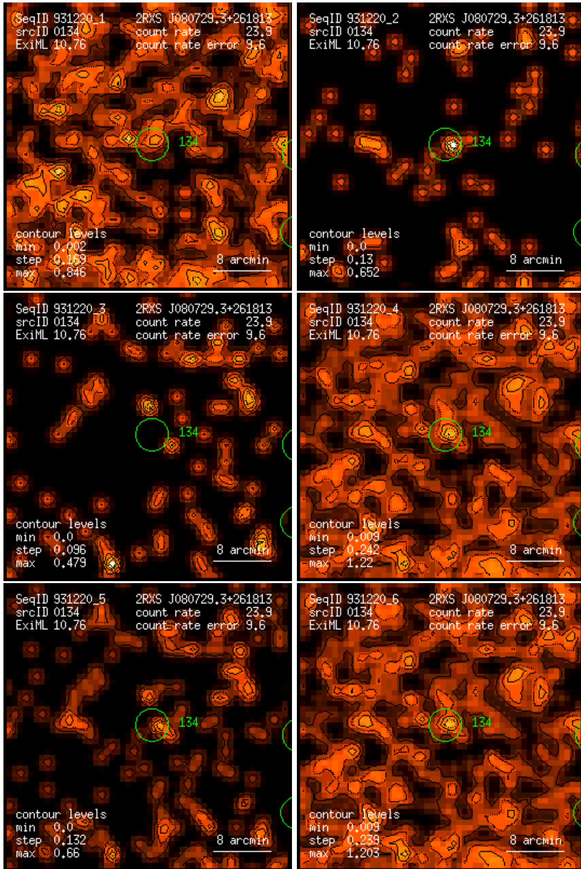
Figure 134: RASS 931220: detection 0134: band rate images, Gaussian filter: (1) PSPC channels 11 – 41, (2) 52 – 90, (3) 91 – 201, (4) 11 – 235, (5) 52 – 201, (6) 11 – 201. Broad band rates in counts/ks. Band rate contour levels in counts/ks/arcmin 2 .
