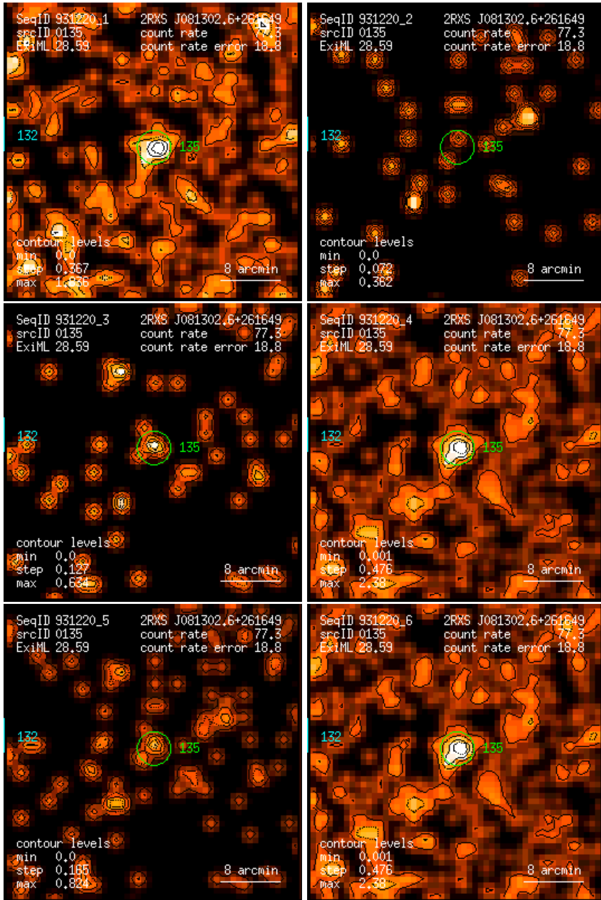
Figure 135: RASS 931220: detection 0135: band rate images, Gaussian filter: (1) PSPC channels 11 – 41, (2) 52 – 90, (3) 91 – 201, (4) 11 – 235, (5) 52 – 201, (6) 11 – 201. Broad band rates in counts/ks. Band rate contour levels in counts/ks/arcmin 2 .
