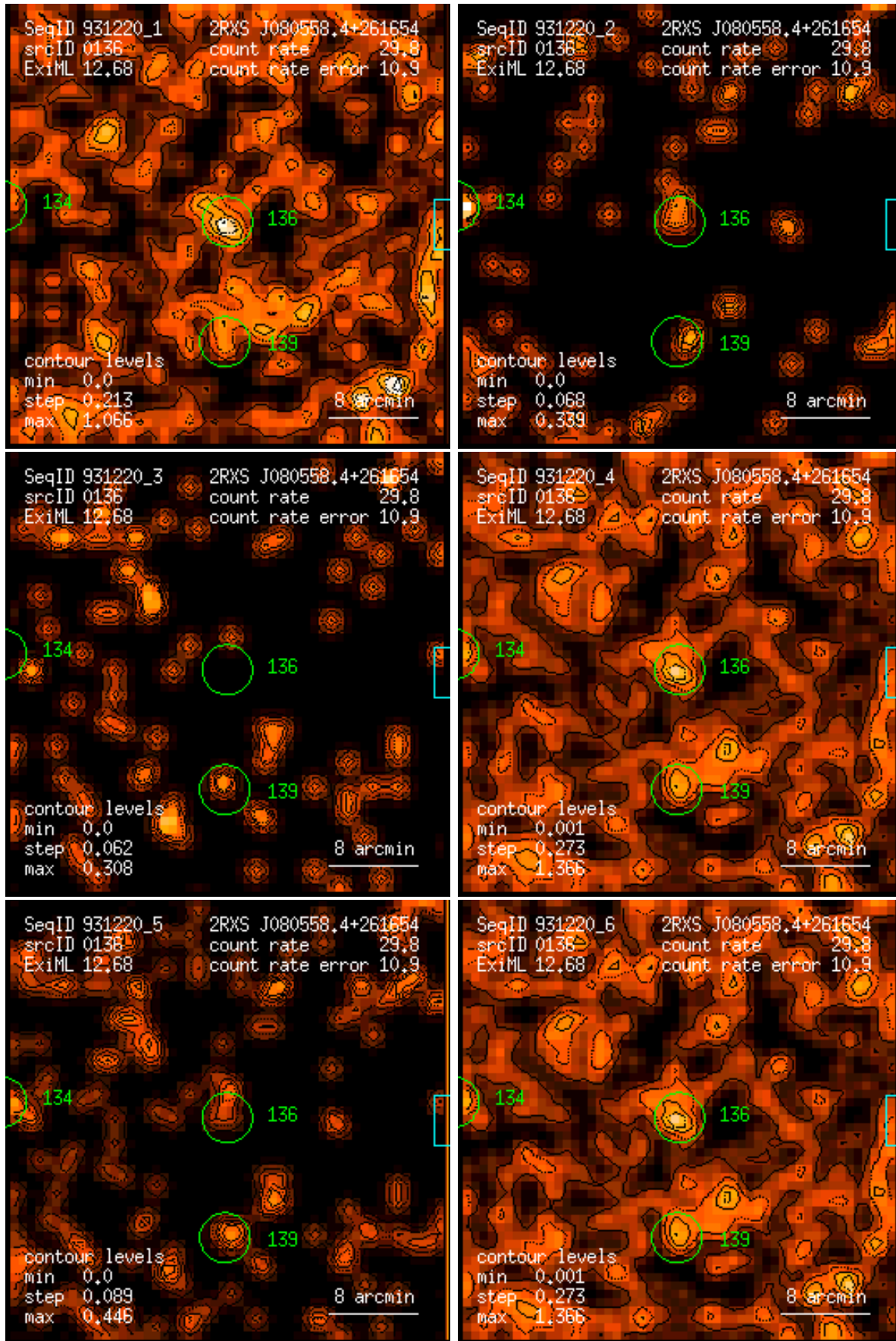
Figure 136: RASS 931220: detection 0136: band rate images, Gaussian filter: (1) PSPC channels 11 – 41, (2) 52 – 90, (3) 91 – 201, (4) 11 – 235, (5) 52 – 201, (6) 11 – 201. Broad band rates in counts/ks. Band rate contour levels in counts/ks/arcmin 2 .
