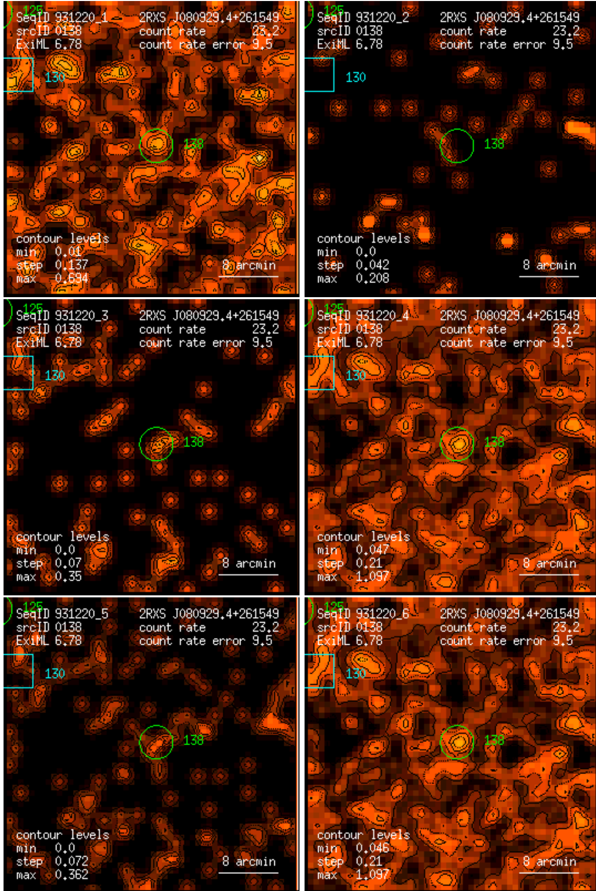
Figure 138: RASS 931220: detection 0138: band rate images, Gaussian filter: (1) PSPC channels 11 – 41, (2) 52 – 90, (3) 91 – 201, (4) 11 – 235, (5) 52 – 201, (6) 11 – 201. Broad band rates in counts/ks. Band rate contour levels in counts/ks/arcmin 2 .
