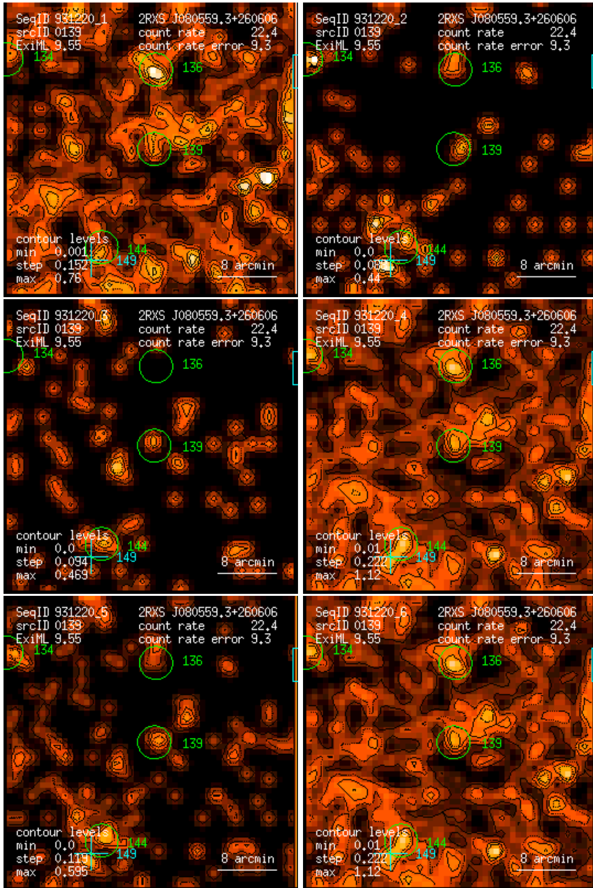
Figure 139: RASS 931220: detection 0139: band rate images, Gaussian filter: (1) PSPC channels 11 – 41, (2) 52 – 90, (3) 91 – 201, (4) 11 – 235, (5) 52 – 201, (6) 11 – 201. Broad band rates in counts/ks. Band rate contour levels in counts/ks/arcmin 2 .
