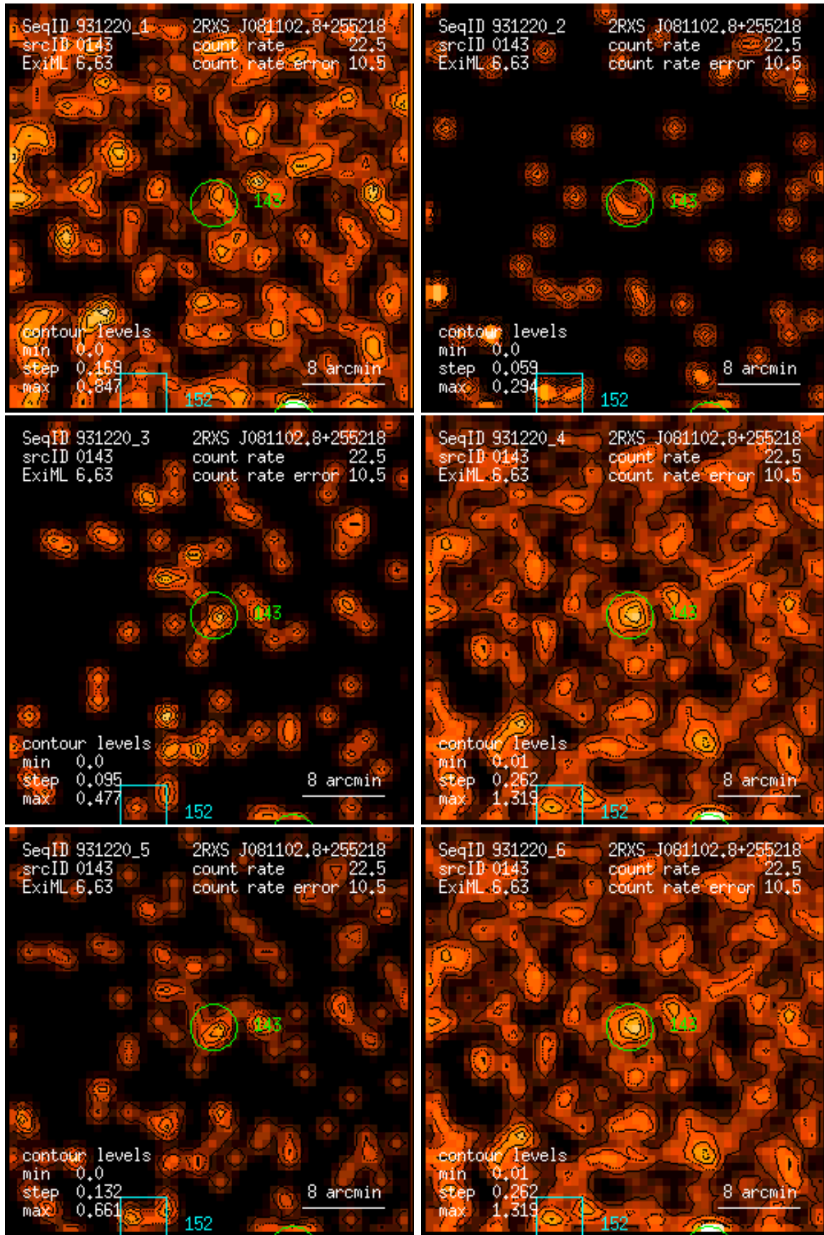
Figure 143: RASS 931220: detection 0143: band rate images, Gaussian filter: (1) PSPC channels 11 – 41, (2) 52 – 90, (3) 91 – 201, (4) 11 – 235, (5) 52 – 201, (6) 11 – 201. Broad band rates in counts/ks. Band rate contour levels in counts/ks/arcmin 2 .
