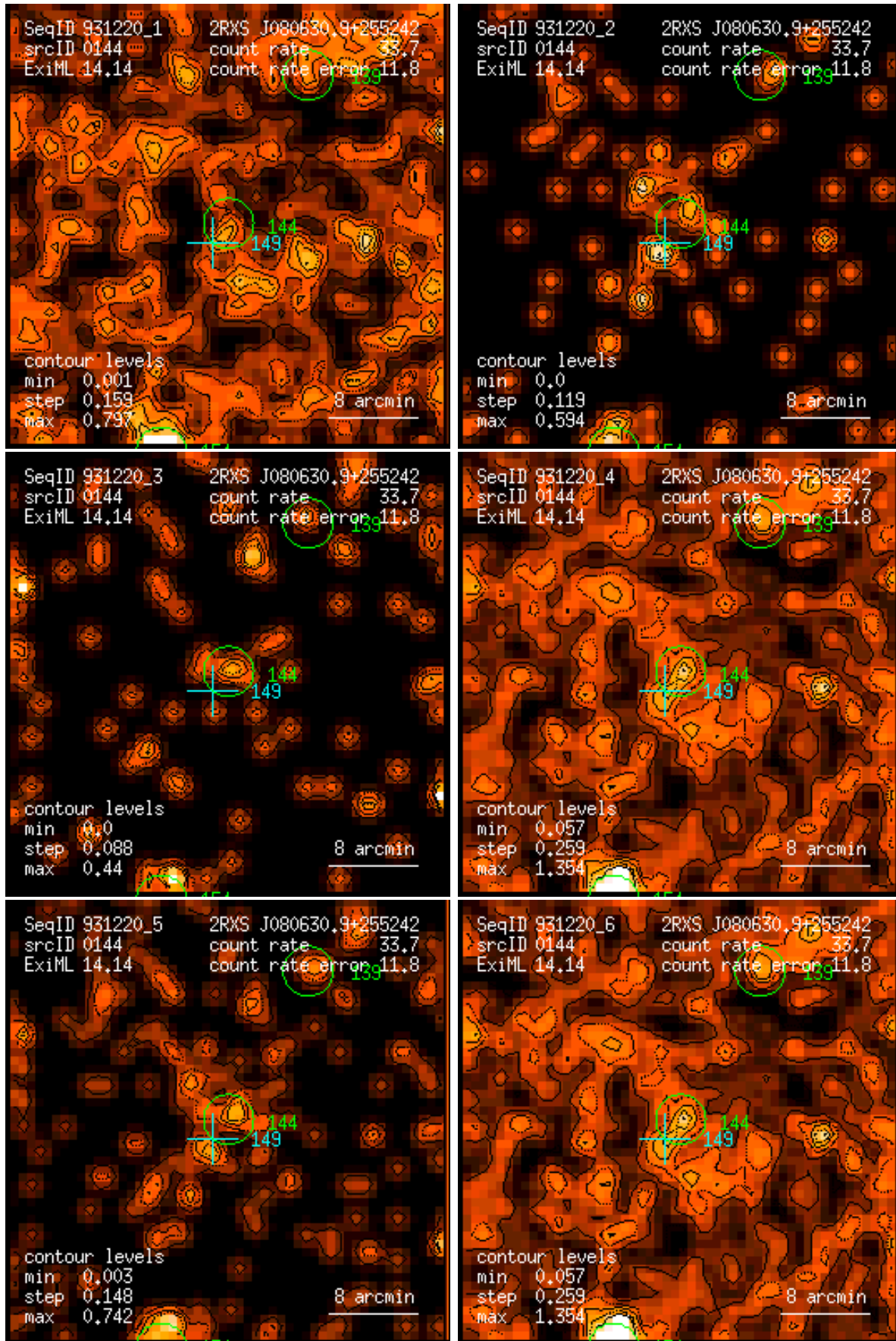
Figure 144: RASS 931220: detection 0144: band rate images, Gaussian filter: (1) PSPC channels 11 – 41, (2) 52 – 90, (3) 91 – 201, (4) 11 – 235, (5) 52 – 201, (6) 11 – 201. Broad band rates in counts/ks. Band rate contour levels in counts/ks/arcmin 2 .
