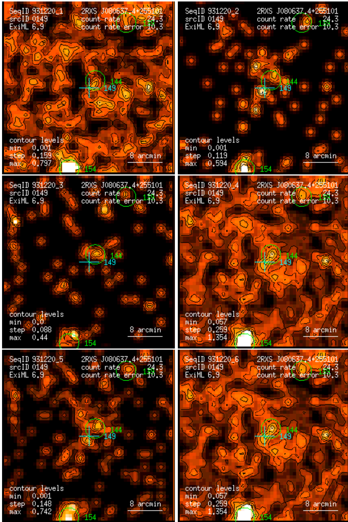
Figure 149: RASS 931220: detection 0149: band rate images, Gaussian filter: (1) PSPC channels 11 – 41, (2) 52 – 90, (3) 91 – 201, (4) 11 – 235, (5) 52 – 201, (6) 11 – 201. Broad band rates in counts/ks. Band rate contour levels in counts/ks/arcmin 2 .
