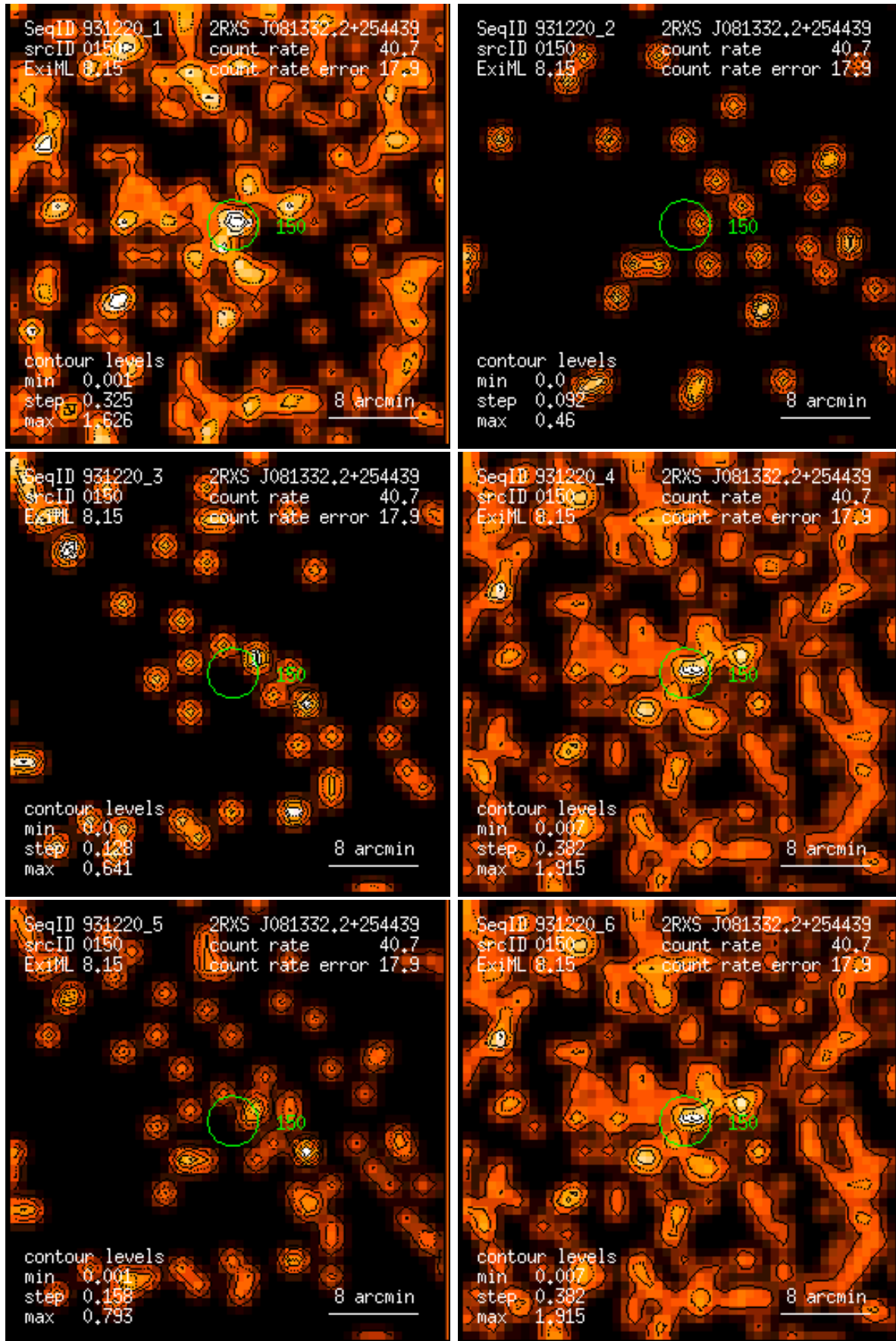
Figure 150: RASS 931220: detection 0150: band rate images, Gaussian filter: (1) PSPC channels 11 – 41, (2) 52 – 90, (3) 91 – 201, (4) 11 – 235, (5) 52 – 201, (6) 11 – 201. Broad band rates in counts/ks. Band rate contour levels in counts/ks/arcmin 2 .
