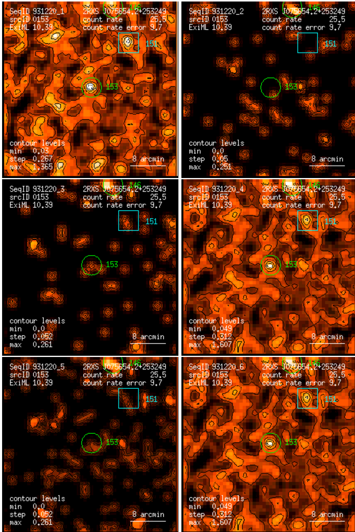
Figure 153: RASS 931220: detection 0153: band rate images, Gaussian filter: (1) PSPC channels 11 – 41, (2) 52 – 90, (3) 91 – 201, (4) 11 – 235, (5) 52 – 201, (6) 11 – 201. Broad band rates in counts/ks. Band rate contour levels in counts/ks/arcmin 2 .
