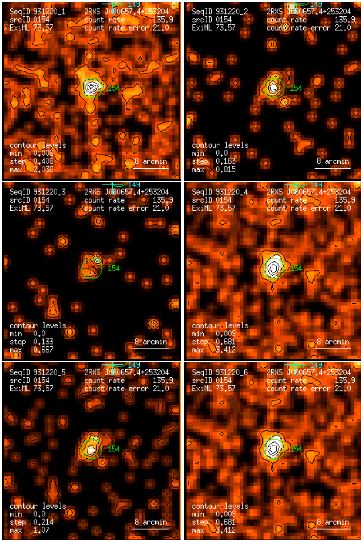
Figure 154: RASS 931220: detection 0154: band rate images, Gaussian filter: (1) PSPC channels 11 – 41, (2) 52 – 90, (3) 91 – 201, (4) 11 – 235, (5) 52 – 201, (6) 11 – 201. Broad band rates in counts/ks. Band rate contour levels in counts/ks/arcmin 2 .
