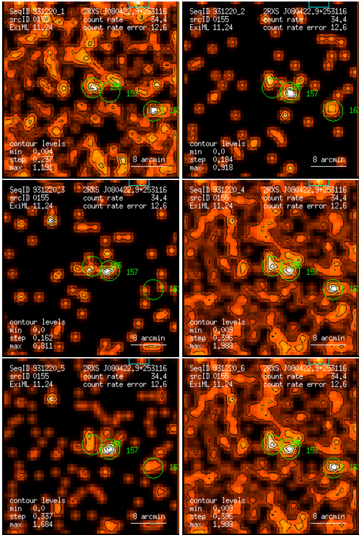
Figure 155: RASS 931220: detection 0155: band rate images, Gaussian filter: (1) PSPC channels 11 – 41, (2) 52 – 90, (3) 91 – 201, (4) 11 – 235, (5) 52 – 201, (6) 11 – 201. Broad band rates in counts/ks. Band rate contour levels in counts/ks/arcmin 2 .
