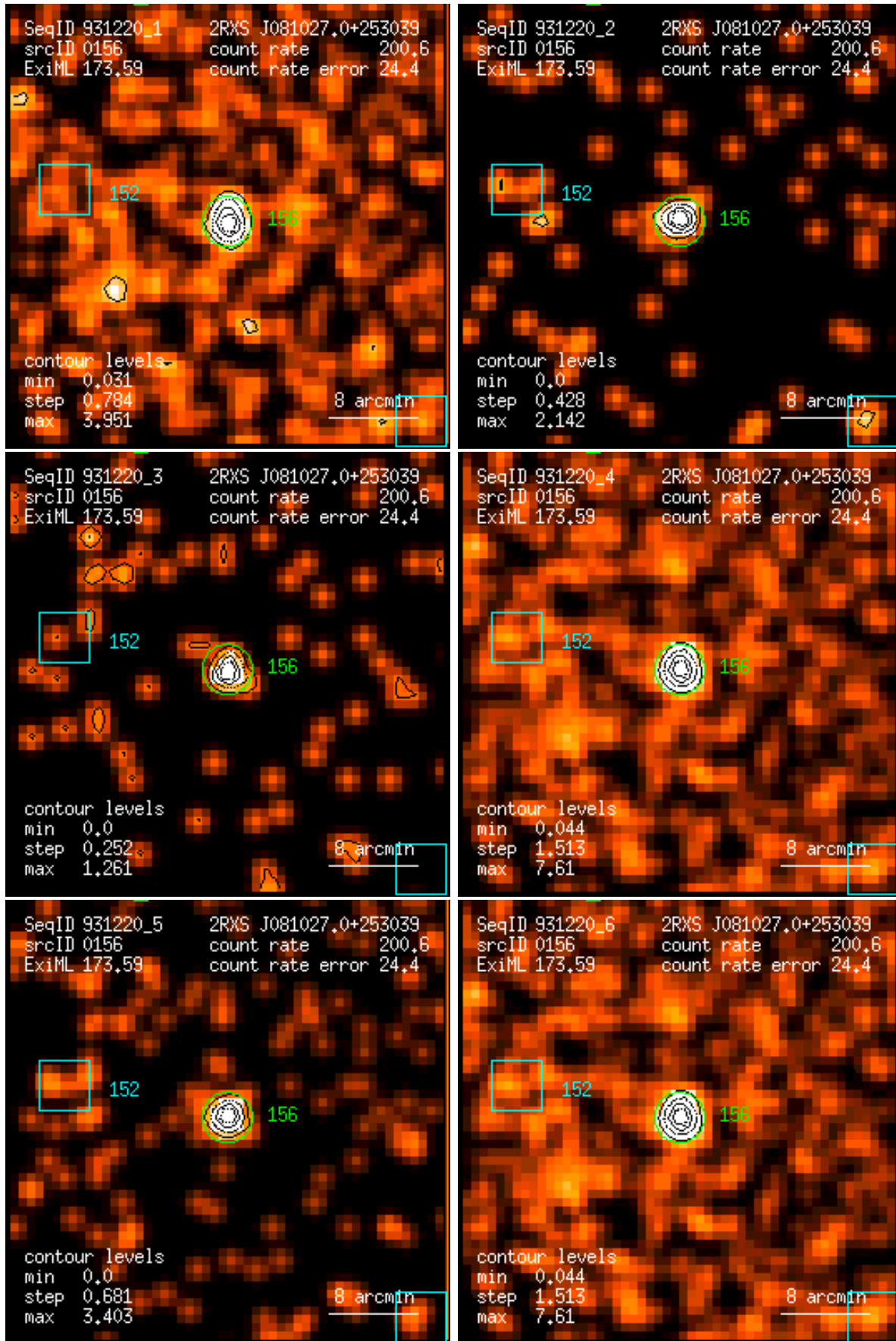
Figure 156: RASS 931220: detection 0156: band rate images, Gaussian filter: (1) PSPC channels 11 – 41, (2) 52 – 90, (3) 91 – 201, (4) 11 – 235, (5) 52 – 201, (6) 11 – 201. Broad band rates in counts/ks. Band rate contour levels in counts/ks/arcmin 2 .
