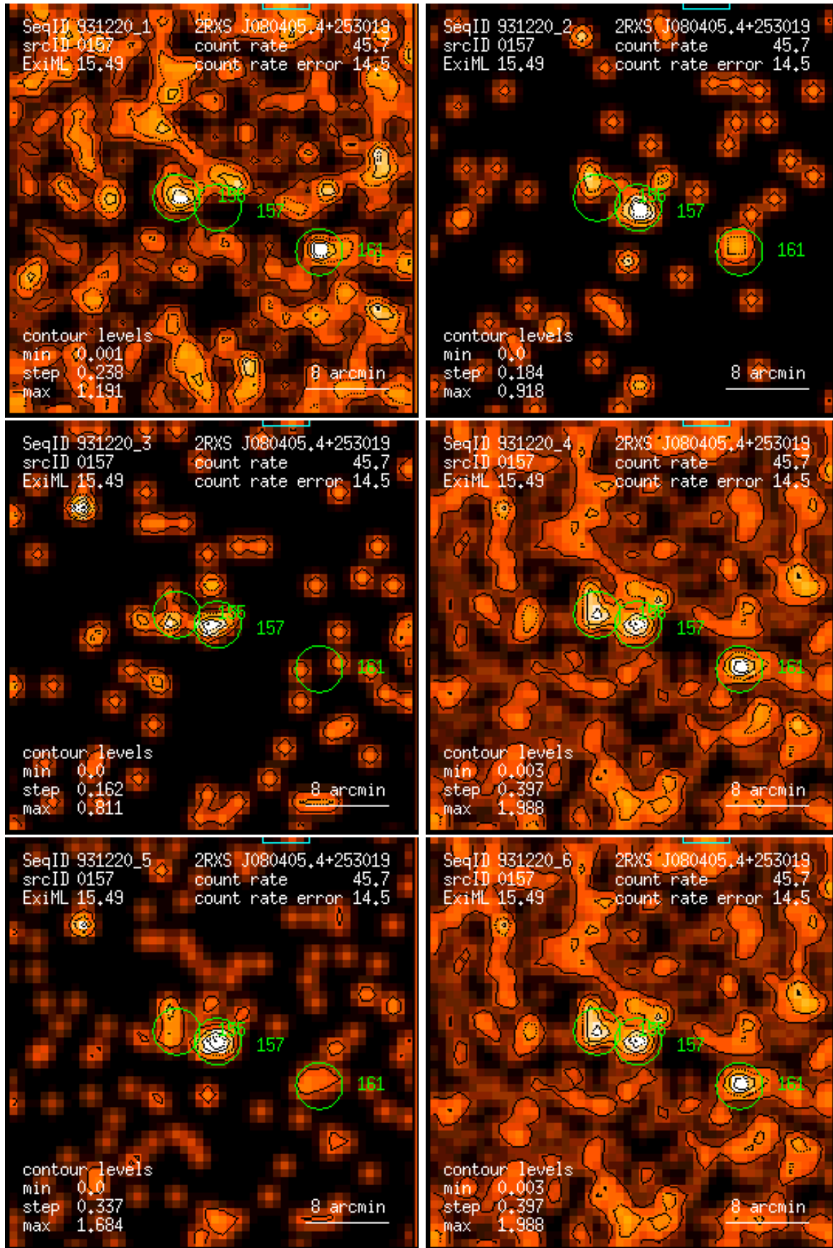
Figure 157: RASS 931220: detection 0157: band rate images, Gaussian filter: (1) PSPC channels 11 – 41, (2) 52 – 90, (3) 91 – 201, (4) 11 – 235, (5) 52 – 201, (6) 11 – 201. Broad band rates in counts/ks. Band rate contour levels in counts/ks/arcmin 2 .
