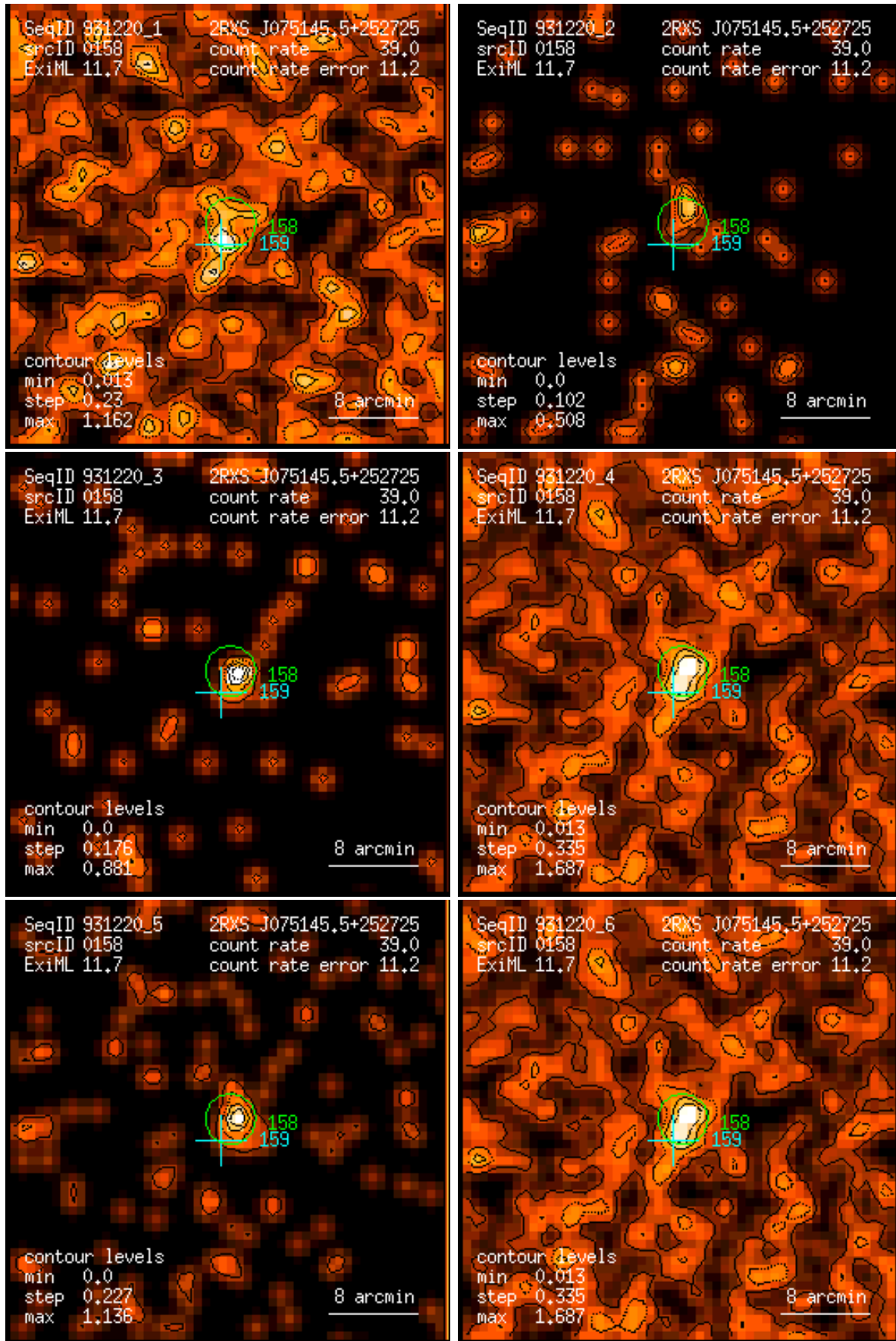
Figure 158: RASS 931220: detection 0158: band rate images, Gaussian filter: (1) PSPC channels 11 – 41, (2) 52 – 90, (3) 91 – 201, (4) 11 – 235, (5) 52 – 201, (6) 11 – 201. Broad band rates in counts/ks. Band rate contour levels in counts/ks/arcmin 2 .
