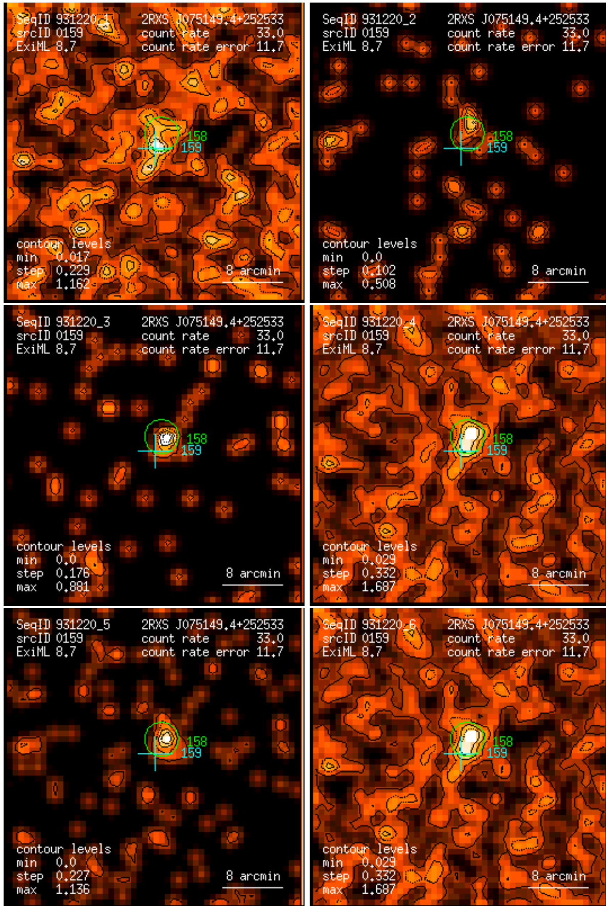
Figure 159: RASS 931220: detection 0159: band rate images, Gaussian filter: (1) PSPC channels 11 – 41, (2) 52 – 90, (3) 91 – 201, (4) 11 – 235, (5) 52 – 201, (6) 11 – 201. Broad band rates in counts/ks. Band rate contour levels in counts/ks/arcmin 2 .
