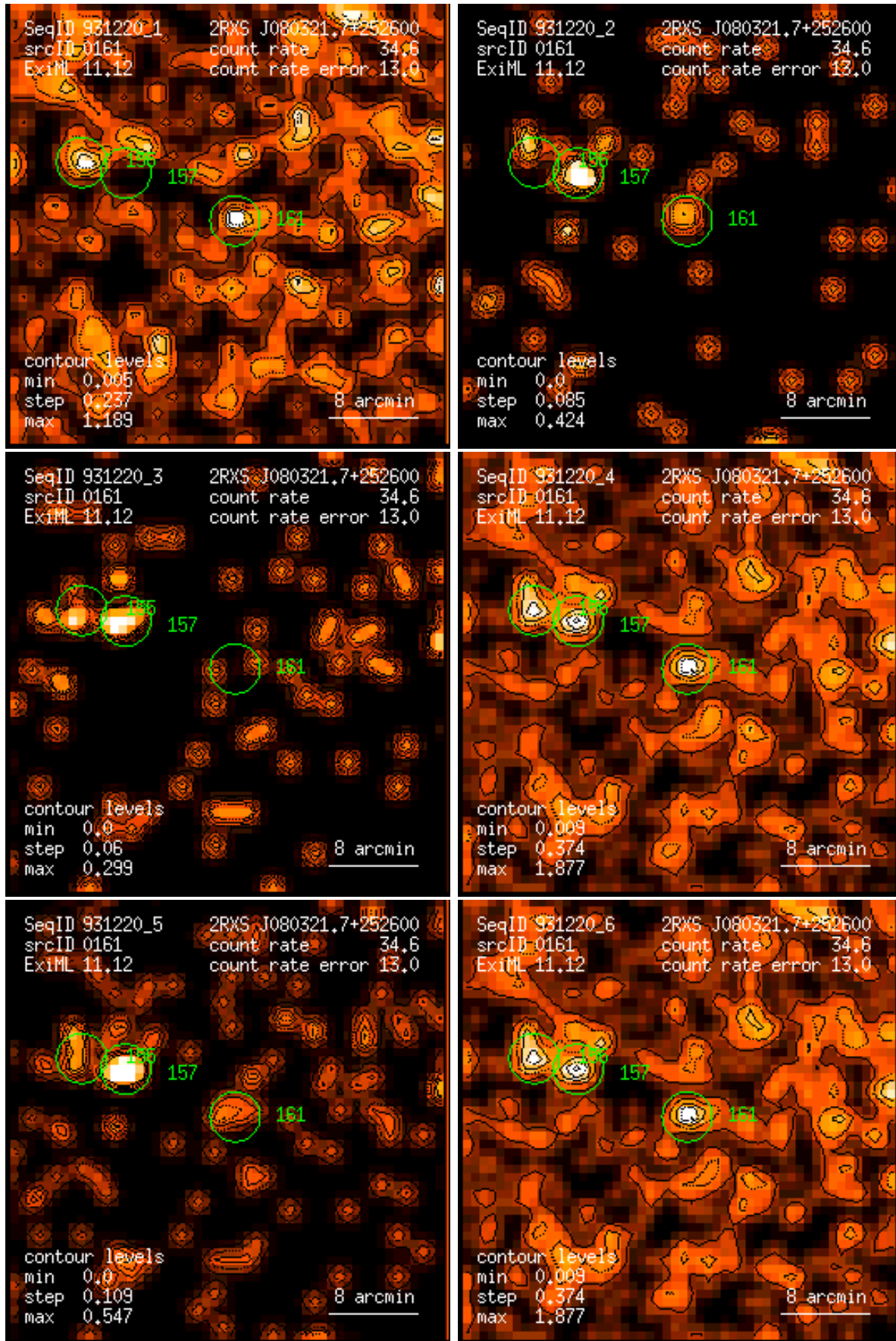
Figure 161: RASS 931220: detection 0161: band rate images, Gaussian filter: (1) PSPC channels 11 – 41, (2) 52 – 90, (3) 91 – 201, (4) 11 – 235, (5) 52 – 201, (6) 11 – 201. Broad band rates in counts/ks. Band rate contour levels in counts/ks/arcmin 2 .
